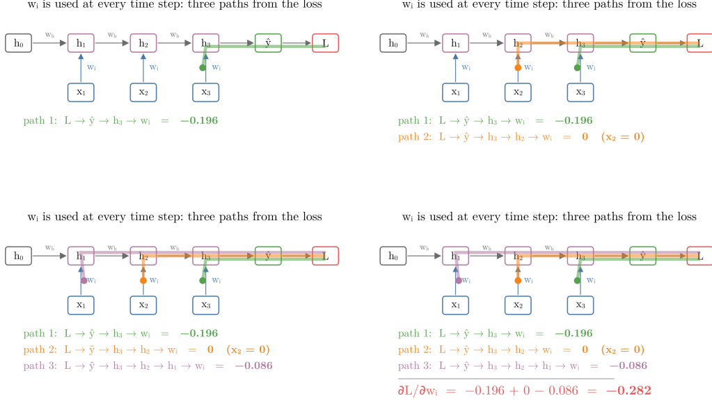
Figure 4: The three paths from the loss back to the shared input weight w_i , traced one at a time: green through h_3 only, orange through h_3 and h_2 , purple through h_3 , h_2 and h_1 . The numbers are the path products of the one-node example (section 6.3); their sum is the gradient
