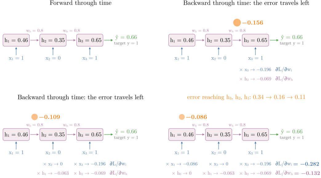
Figure 6: BPTT on the one-node example as one backward walk. The orange disc is the error reaching each hidden state; at each step it is multiplied by the tanh slope, drops one term into \partial L/\partial w_i (times x_t ) and one into \partial L/\partial w_h (times h_{t-1} ), then is multiplied by w_h to reach the step before
