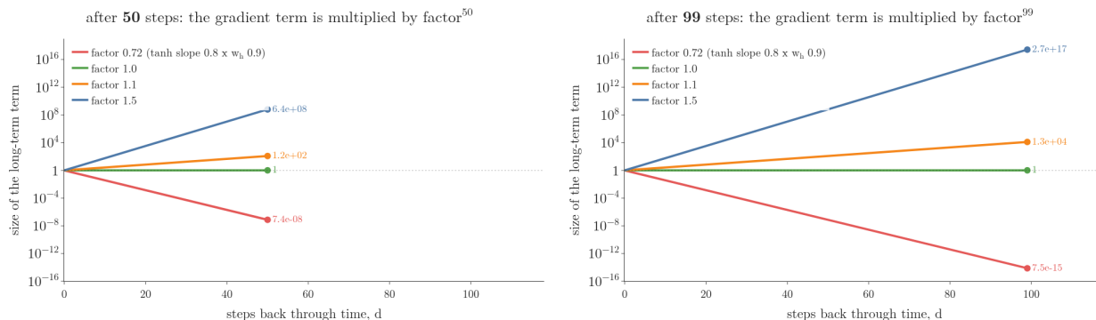
Figure 6: The same factor multiplied once per step back through time, for four factors (log scale). Below 1 the product falls towards 0 (vanishing); at 1 it stays; above 1 it grows without limit (exploding). The orange and blue lines are the two examples above; the red line is the 0.72^{99} of section 4.3
