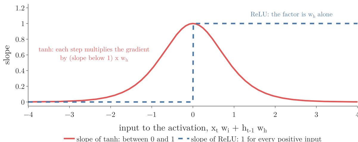
Figure 5: The slope of the activation, which multiplies w_h at every backward step. tanh’s slope (red) is 1 only at 0 and smaller everywhere else, so each step shrinks the gradient. ReLU’s slope (blue) is exactly 1 for every positive input, so the factor is w_h alone
