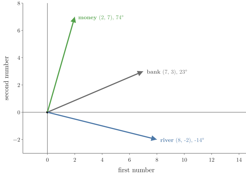
Figure 2: The hand-picked embeddings as arrows from the origin, with the angle of each. “Money” points up, “river” slightly down, and “bank” in between
