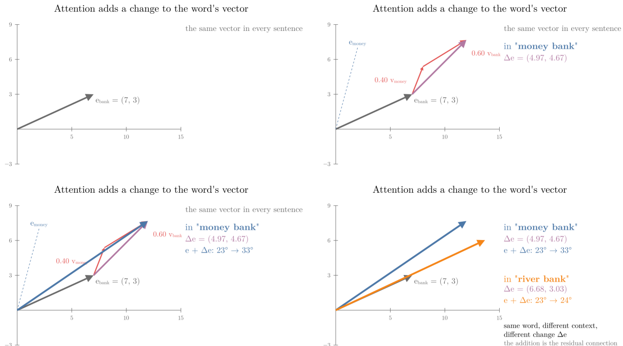
Figure 6: The attention output as a change added to the word’s vector. The weighted value vectors (red) are placed at the tip of e_{bank} (grey); their sum is \Delta e (purple); e_{bank} + \Delta e is the new vector, blue for “money bank” and orange for “river bank”
