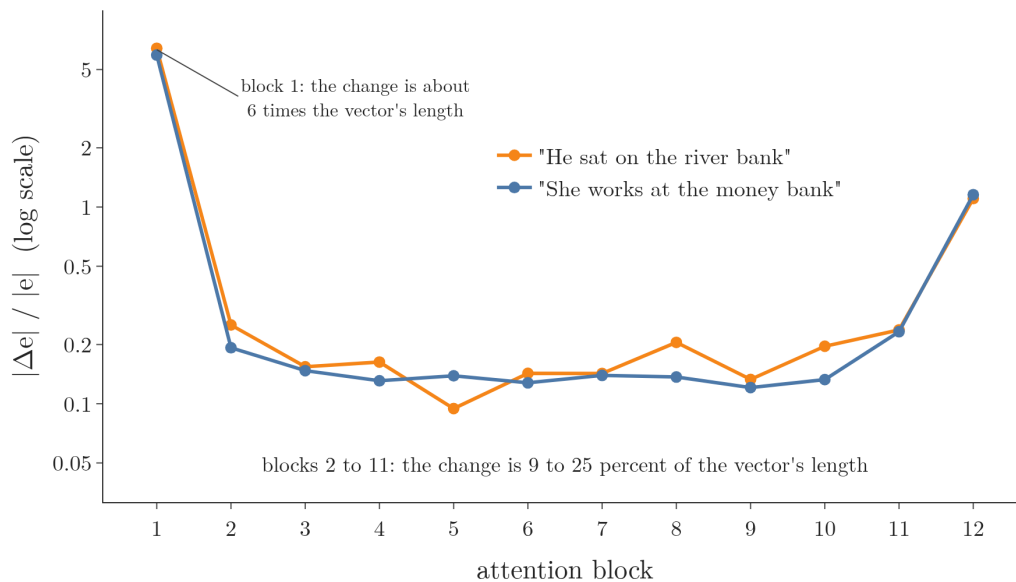
Figure 7: GPT-2 small: the length of the change added by each attention block, relative to the vector it is added to, for the last token “bank” of two real sentences (log scale)
