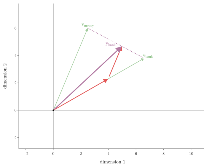
Figure 5: Step 3 as a still: the shrunk value vectors (red) placed tip to tail; their sum is y_{\text{bank}} (purple), on the dotted line between the two value vectors
