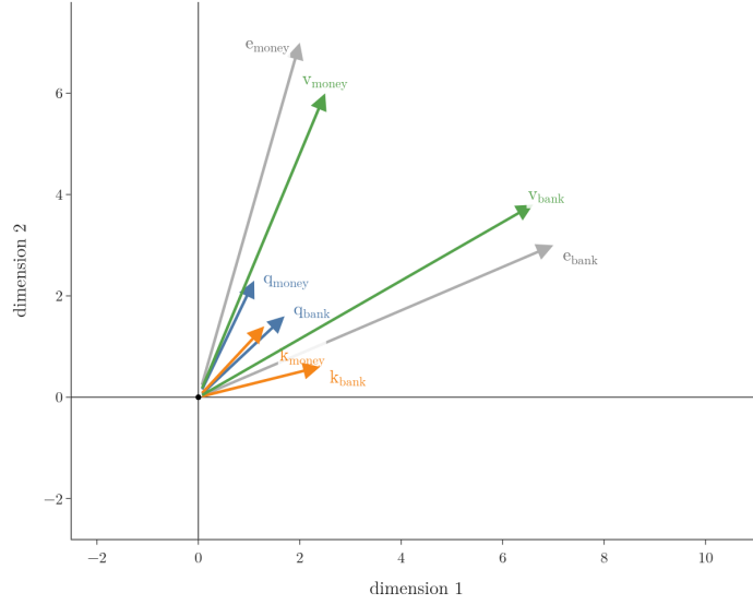
Figure 3: Step 1 as a still: the grey embeddings and their query (blue), key (orange) and value (green) vectors
