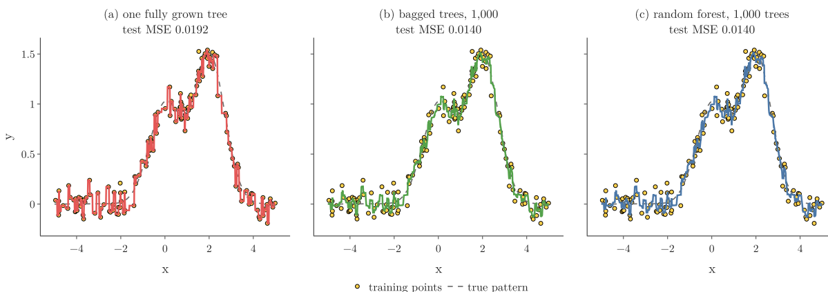
Figure 4: Two bumps plus noise: (a) one fully grown regression tree; (b) bagging with 1,000 fully grown trees; (c) a random forest of 1,000 trees. The dashed curve is the true pattern
