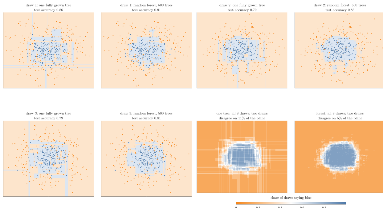
Figure 3: The circles data drawn eight times. Each frame: one fully grown tree (left) and a random forest of 500 trees (right) trained on that draw, with test accuracy. Last frame: the share of the eight surfaces that say blue; white means the draws disagree
