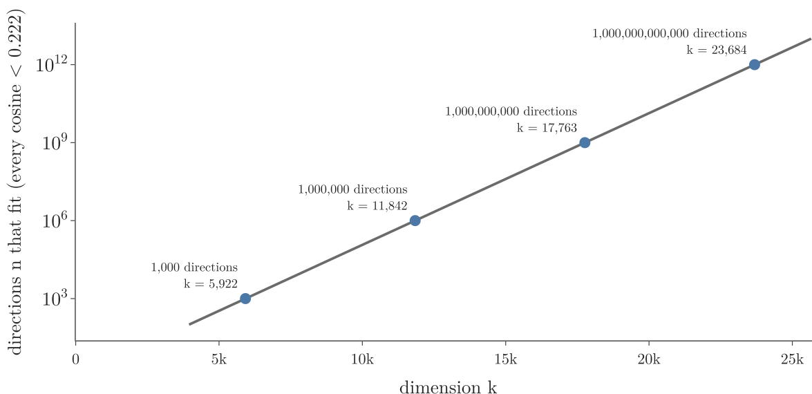
Figure 5: The Johnson–Lindenstrauss guarantee with \varepsilon = 0.1 : the number of directions that fit, every cosine below 0.222, against the dimension. On a log scale the line is straight: the count grows exponentially with the dimension
