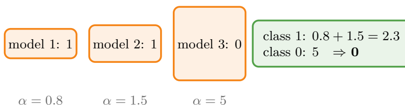
Figure 4: Equal against weighted votes. Bagging: four models answer 1, 1, 0, 1 with weight 1 each, so 1 wins three votes to one. Boosting: three models answer 1, 1, 0 with alphas 0.8, 1.5 and 5 (box height), so 0 wins, 5 to 2.3
