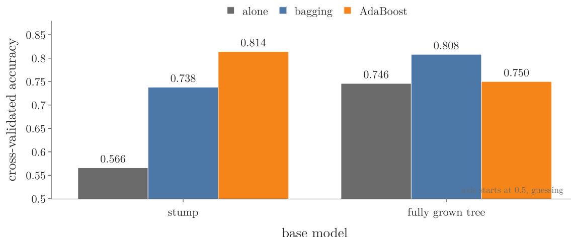
Figure 2: The table as bars. Boosting lifts the stump most (0.566 to 0.814); bagging lifts the fully grown tree most (0.746 to 0.808)
