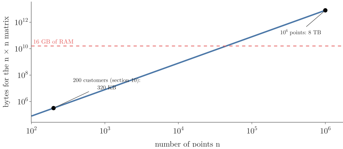
Figure 9: Memory for the full proximity matrix at 8 bytes per distance. The 200 customers of section 10 need 320 KB; a million points need 8 TB, far above 16 GB of RAM. Both axes are logarithmic
