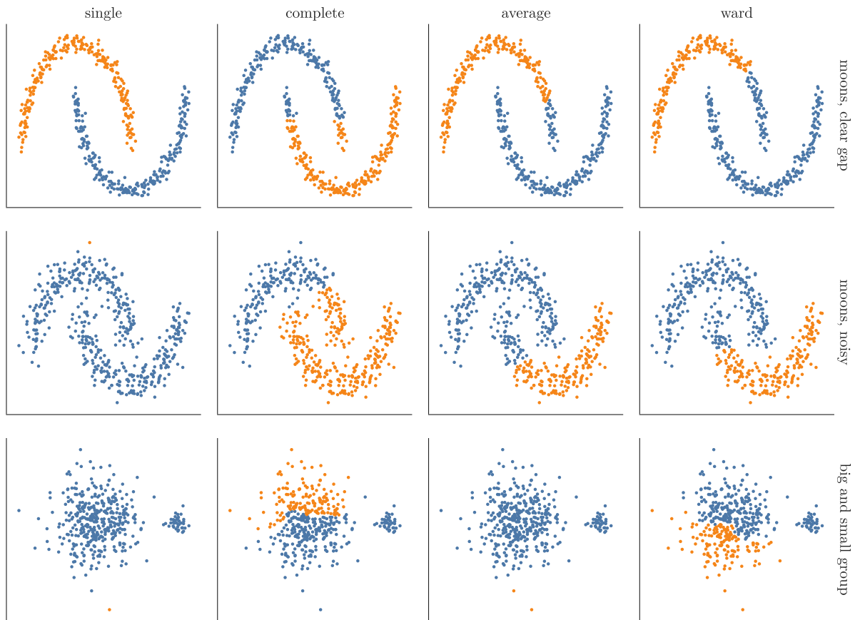
Figure 6: Single, complete, average and Ward linkage (2 clusters) on moons with a clear gap, noisy moons, and a big and a small group
