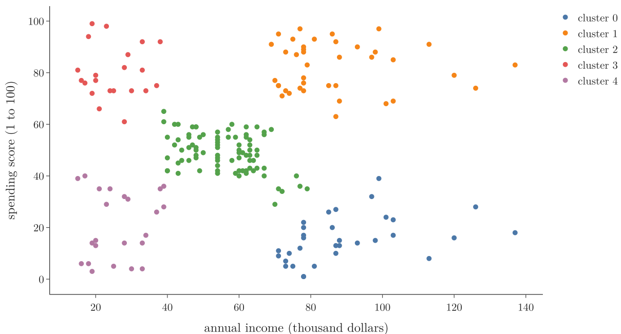
Figure 8: The 200 customers in the 5 clusters found by Ward linkage
