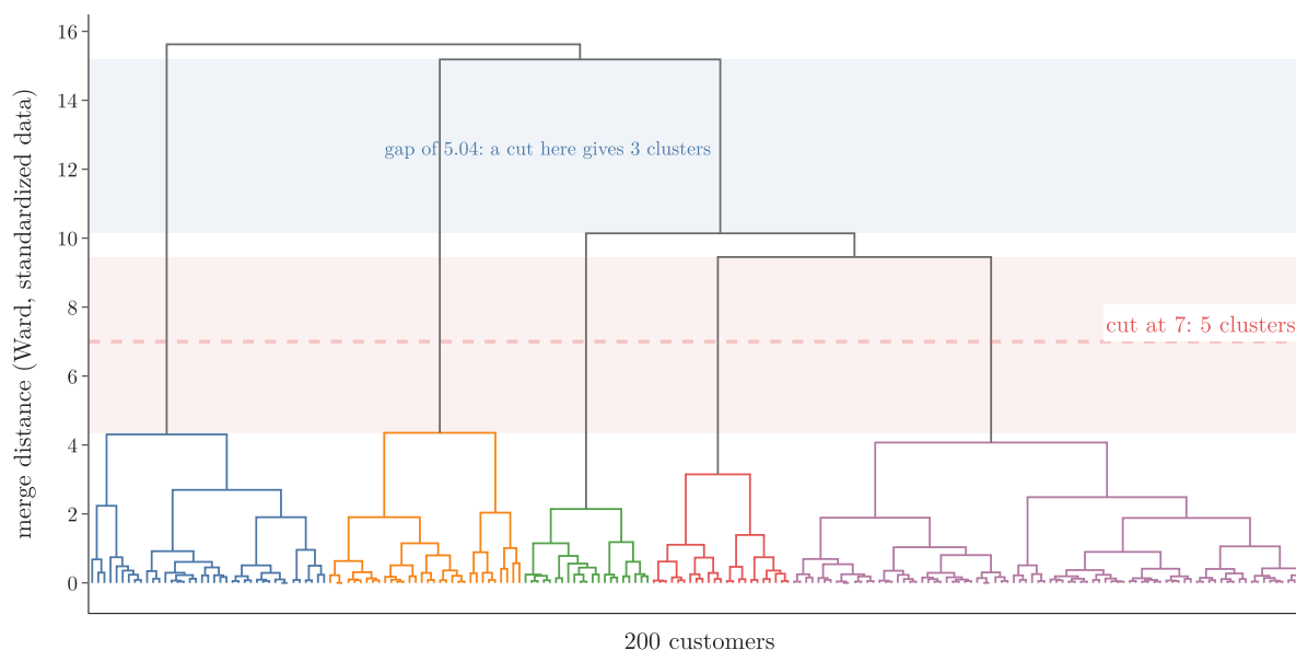
Figure 7: Ward dendrogram of the 200 customers (standardized features); the cut at 7 gives 5 clusters
