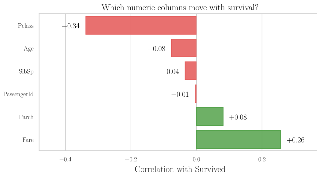
Figure 8: Correlation of each numerical column with Survived
