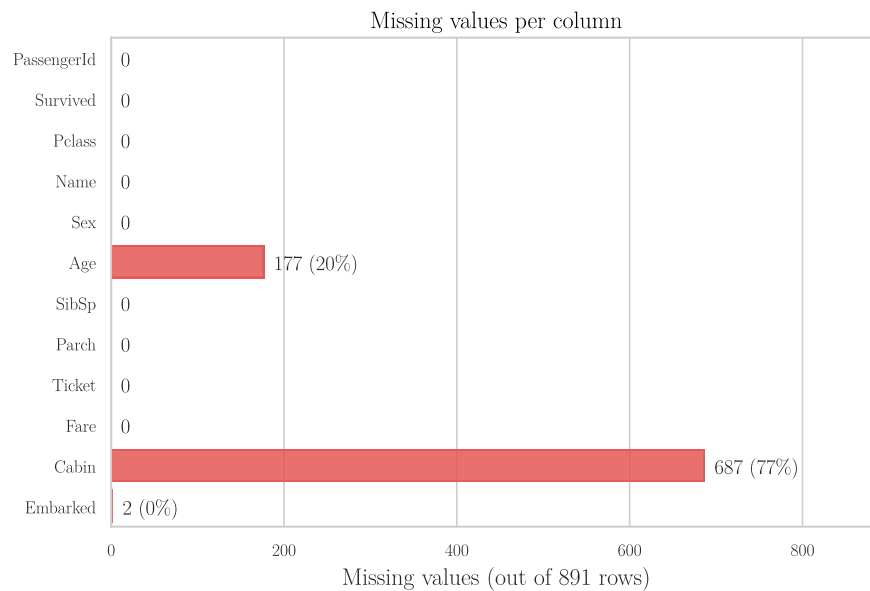
Figure 4: Missing values in each column of the Titanic data
