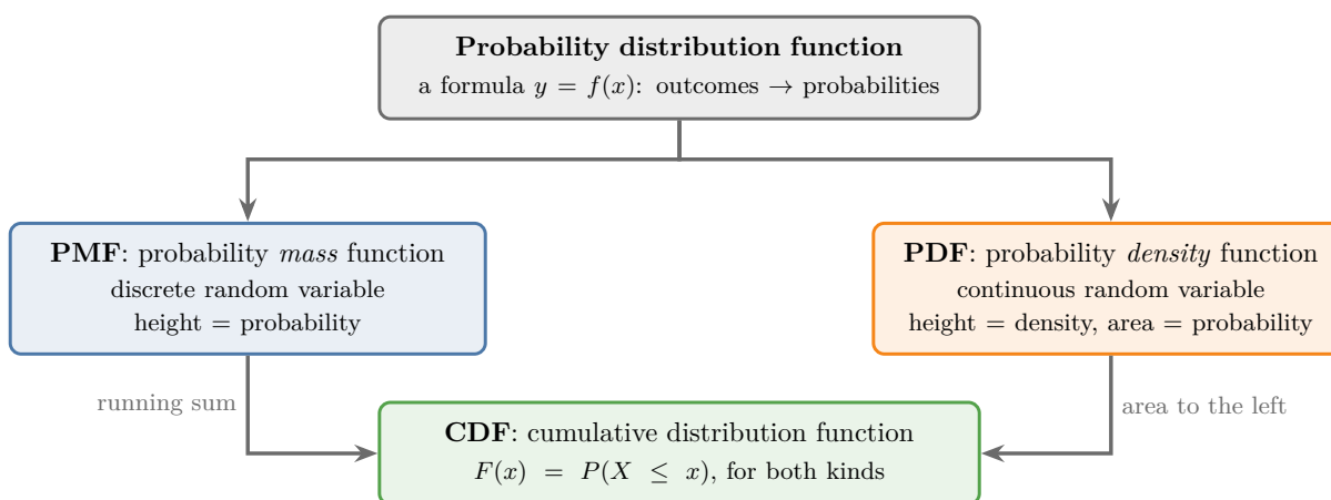
Figure 1: The family of probability distribution functions
