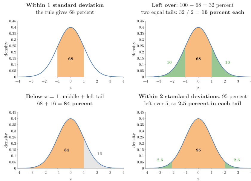
Figure 8: Tail areas from the rule: the middle 68 percent leaves 32, split into two tails of 16; below z = 1 lies 68 + 16 = 84 percent; beyond 2 standard deviations each tail holds 2.5 percent. Idea after Khan Academy, “ck12.org exercise: Standard normal distribution and the empirical rule”
