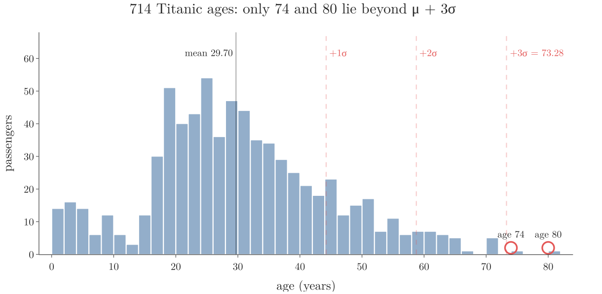
Figure 9: The 714 Titanic ages with the mean and the +1, +2 and +3 standard deviation lines. Only the passengers aged 74 and 80 (circled) lie beyond 73.28.
