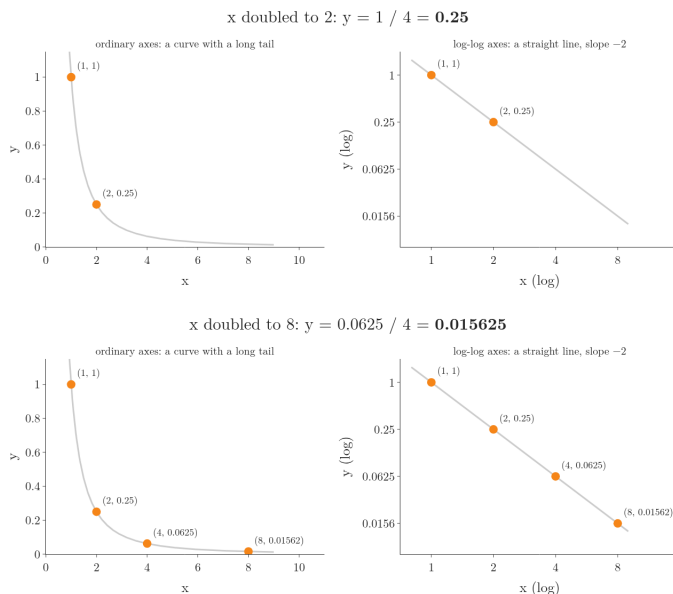
Figure 2: The power law y = x^{-2} at x = 1, 2, 4 and 8 : each doubling divides y by 4 . Left: ordinary axes. Right: log-log axes, where the points lie on a straight line with slope -2 .
