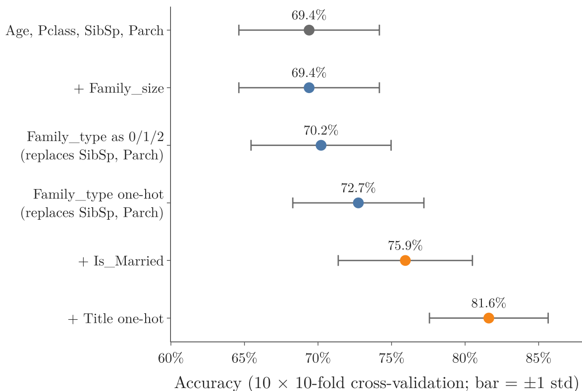
Figure 8: Cross-validated accuracy for each set of features (grey: baseline; blue: construction; orange: splitting)
