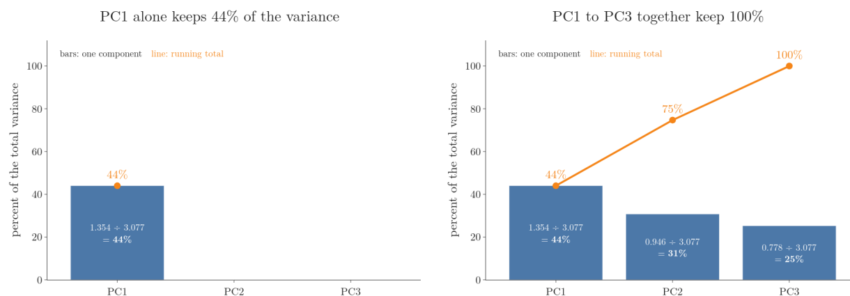
Figure 9: The scree plot of the 3-feature example, built one component at a time. Bars: eigenvalue ÷ sum of eigenvalues. Orange line: the running total.
