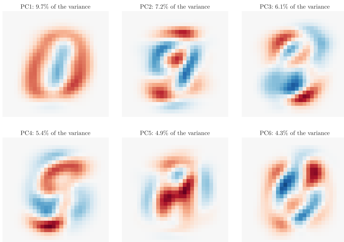
Figure 7: The first six eigenvectors of MNIST, each reshaped to 28 \times 28 (PCA fitted on all 70,000 images). Red pixels count positively, blue negatively. The variance shares, 9.7, 7.2 and 6.1 percent for the first three, match the table within 0.1 point.
