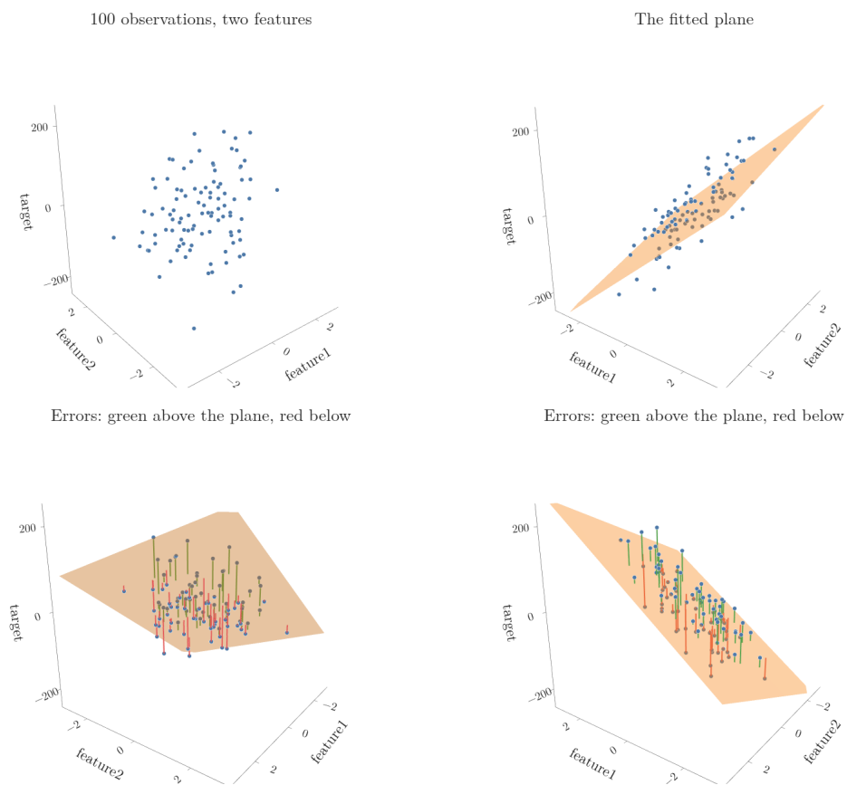
Figure 2: 100 observations in 3D, then the fitted plane, then each observation's error as a stick to the plane (green above, red below), while the view circles once
