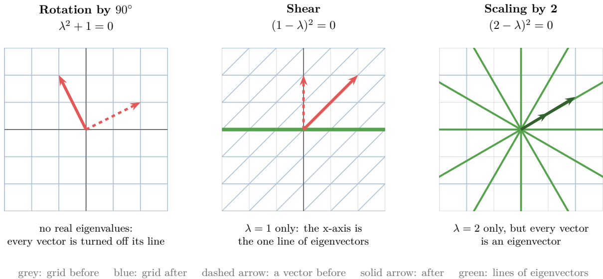
Figure 5: Three transformations with very different eigenvectors
