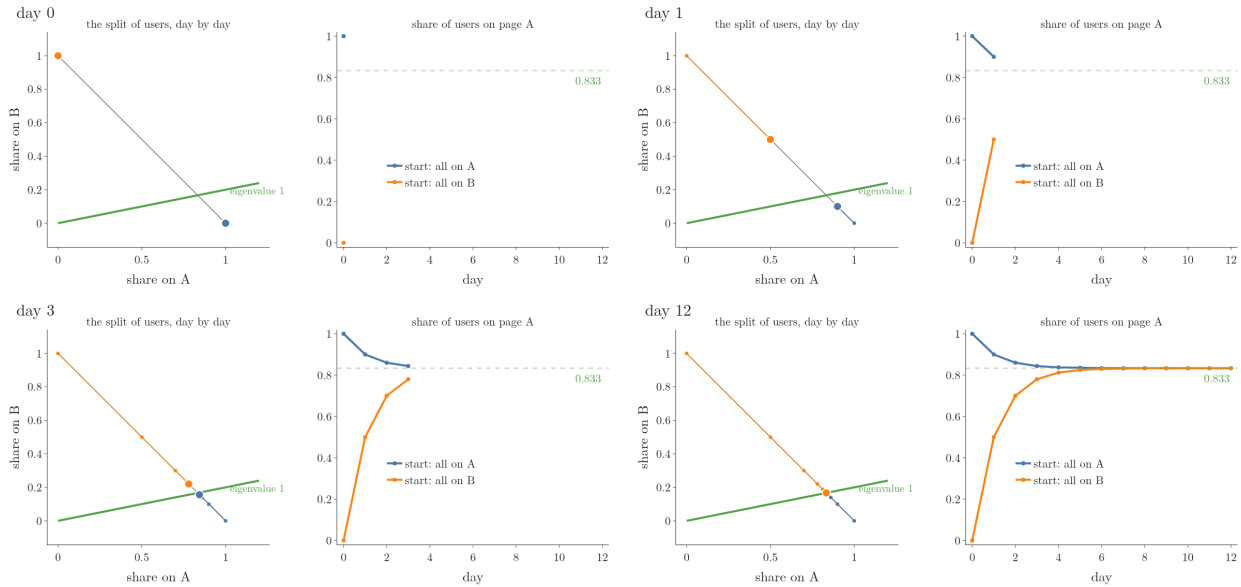
Figure 7: Power iteration with the one-day matrix T . Left: each day's split of users as a point; both starting splits slide onto the green eigenvector of eigenvalue 1. Right: the share of users on page A settles at 0.833 from either start.
