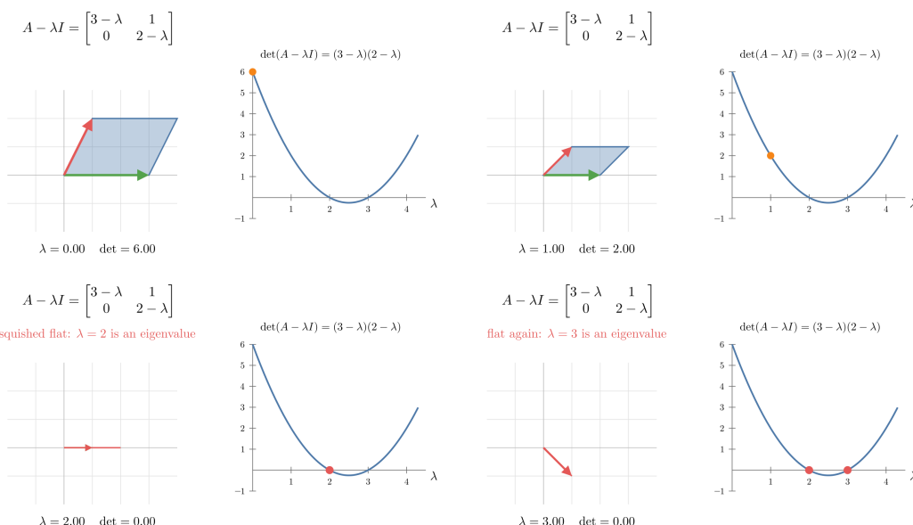
Figure 3: Turning the knob \lambda : A - \lambda I squishes the unit square flat exactly when \lambda is an eigenvalue of A
