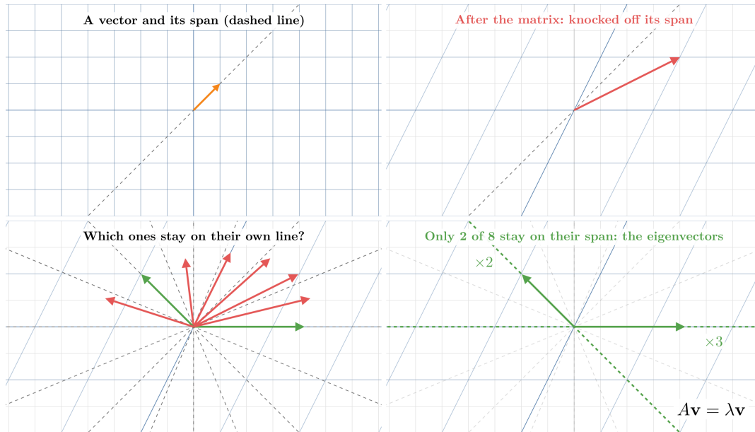
Figure 1: Eight vectors and their spans (dashed) go through A together with the grid; six are knocked off their line (red), only the two eigenvectors stay on it (green), stretched by 3 and by 2
