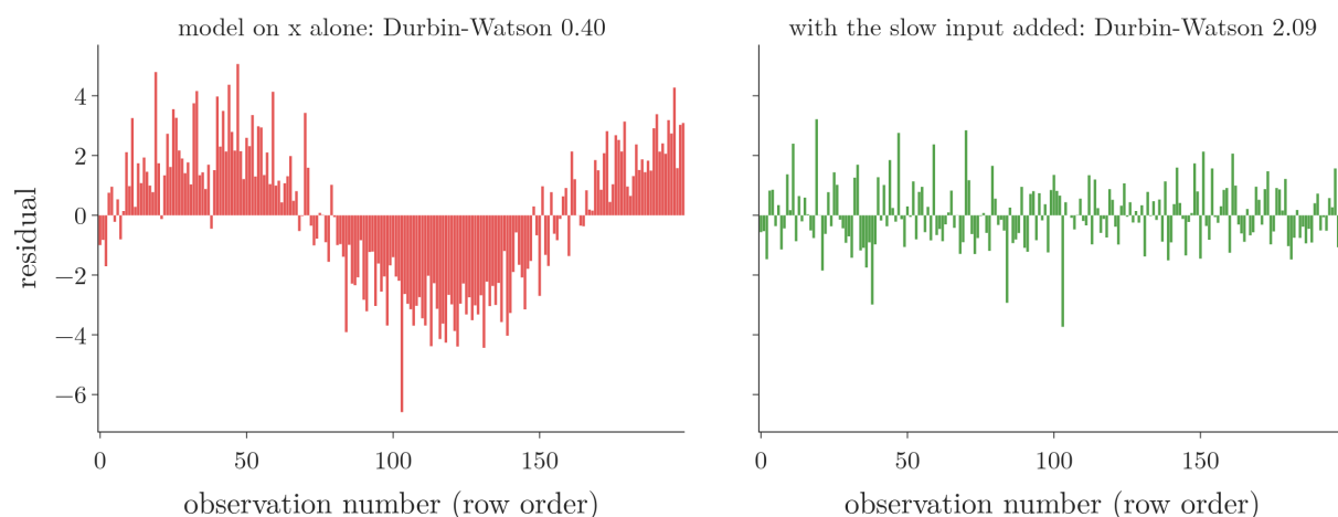
Figure 7: Residuals in row order for data built as y = 2x + 3 \sin(t/25) + \text{noise} . Left: a model on x alone leaves the slow wave in its residuals (Durbin-Watson 0.40). Right: with \sin(t/25) added as a feature, the residuals jump randomly (Durbin-Watson 2.09).
