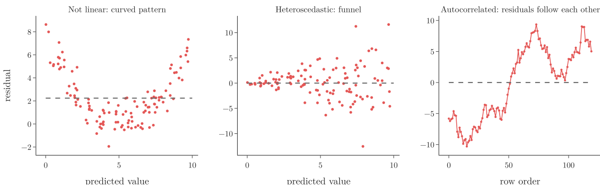
Figure 6: What failed assumptions look like (made-up data)
