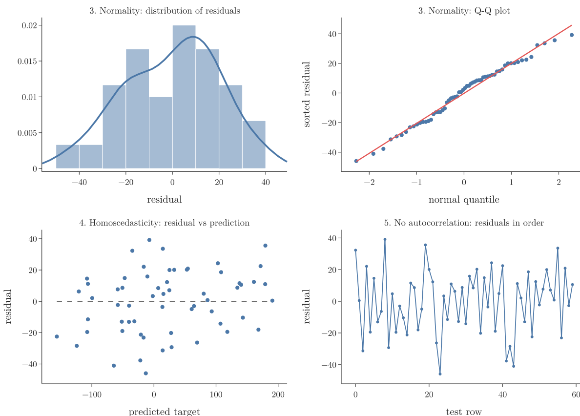
Figure 5: Residual checks for assumptions 3, 4 and 5
