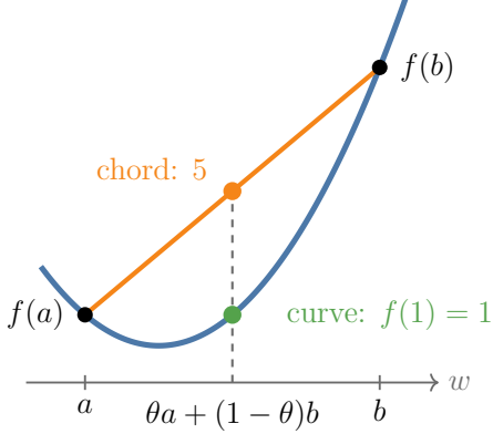
Figure 3: The chord test. Left: for w^2 , the curve at the midpoint (1) is below the chord (5): convex. Right: for g(w) = w^4 - 4w^2 + w , the curve at the midpoint (0) is above the chord (-3.94): non-convex
