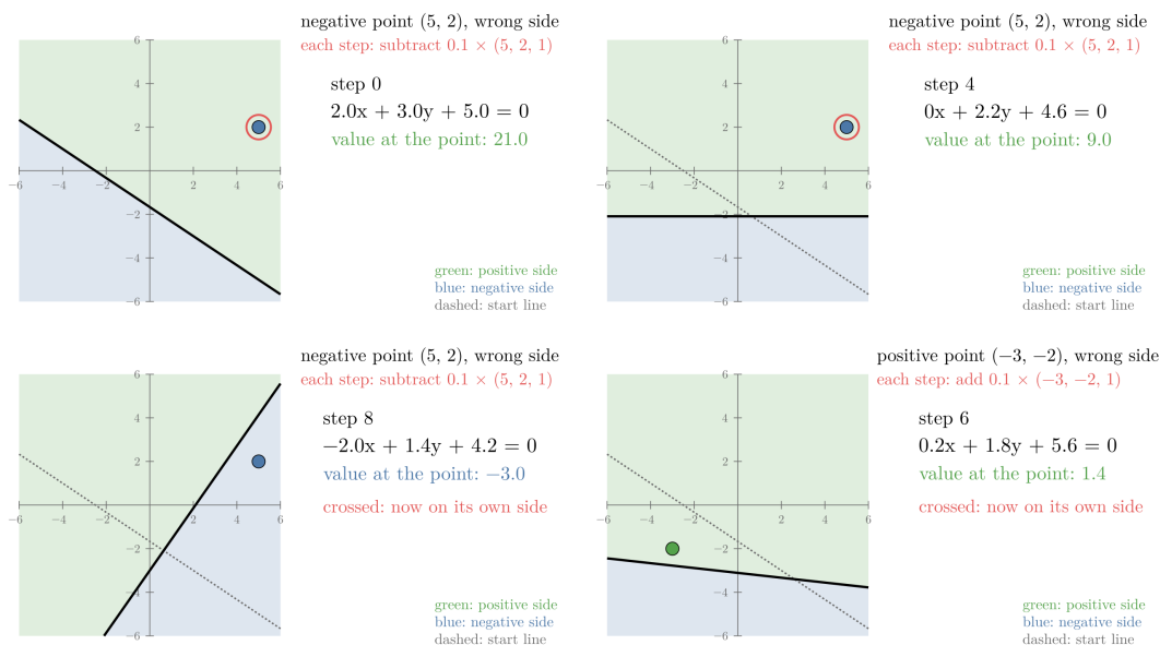
Figure 6: The perceptron trick in small steps, learning rate 0.1. First, the negative point (5, 2) sits on the positive (green) side; each step subtracts 0.1 \times (5, 2, 1) from the coefficients, its value falls by 3 (21, 18, 15, ...), and at step 8 the point is on the negative side. Then the positive point (-3, -2); each step adds 0.1 \times (-3, -2, 1) , its value rises by 1.4 from -7, and it crosses at step 6. The dashed line is the start line 2x + 3y + 5 = 0
