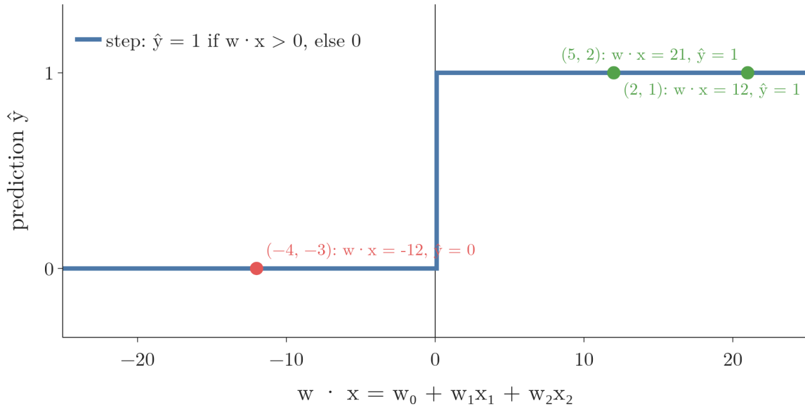
Figure 7: The step function turns w \cdot x into a prediction. With the line 2x + 3y + 5 = 0 : (2, 1) gives 12 and \hat{y} = 1 , (5, 2) gives 21 and \hat{y} = 1 , (-4, -3) gives -12 and \hat{y} = 0 .
