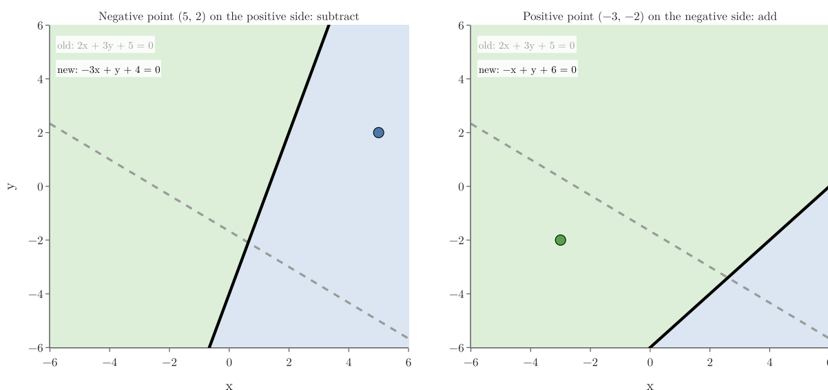
Figure 5: One update for each kind of mistake
