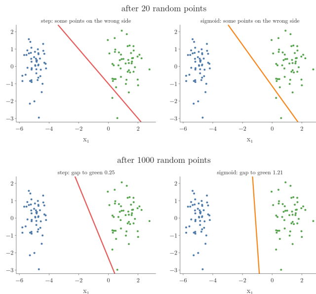
Figure 6: The step perceptron (left) and the sigmoid perceptron (right) trained on the same random points, learning rate 0.1. The step line stops changing after 44 points; the sigmoid line keeps moving away from the green class, ending with a gap of 1.21 against 0.25.
