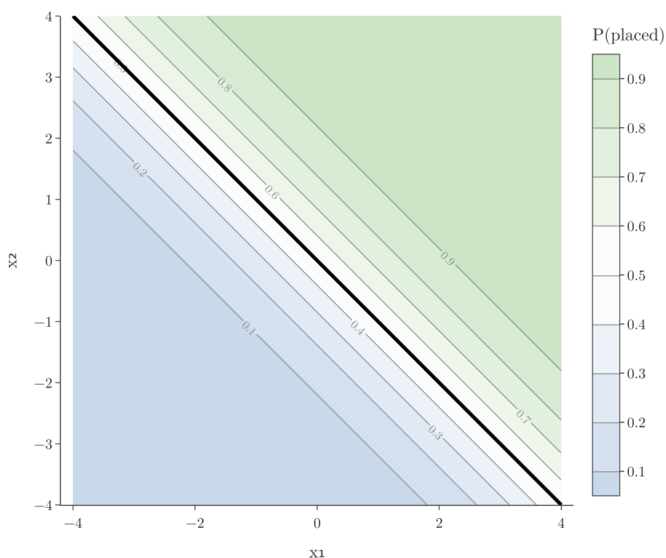
Figure 3: \sigma(w \cdot x) as the probability of being placed
