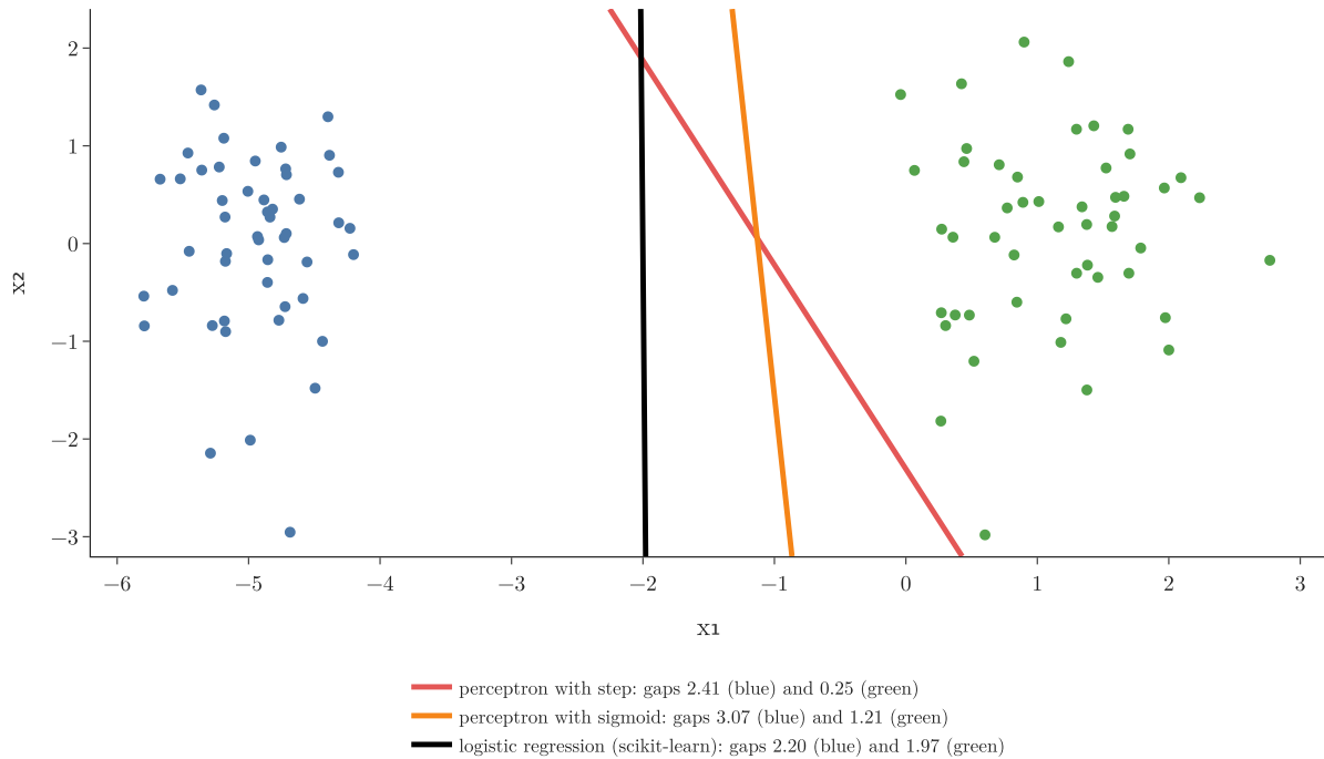
Figure 5: Step perceptron, sigmoid perceptron and logistic regression
