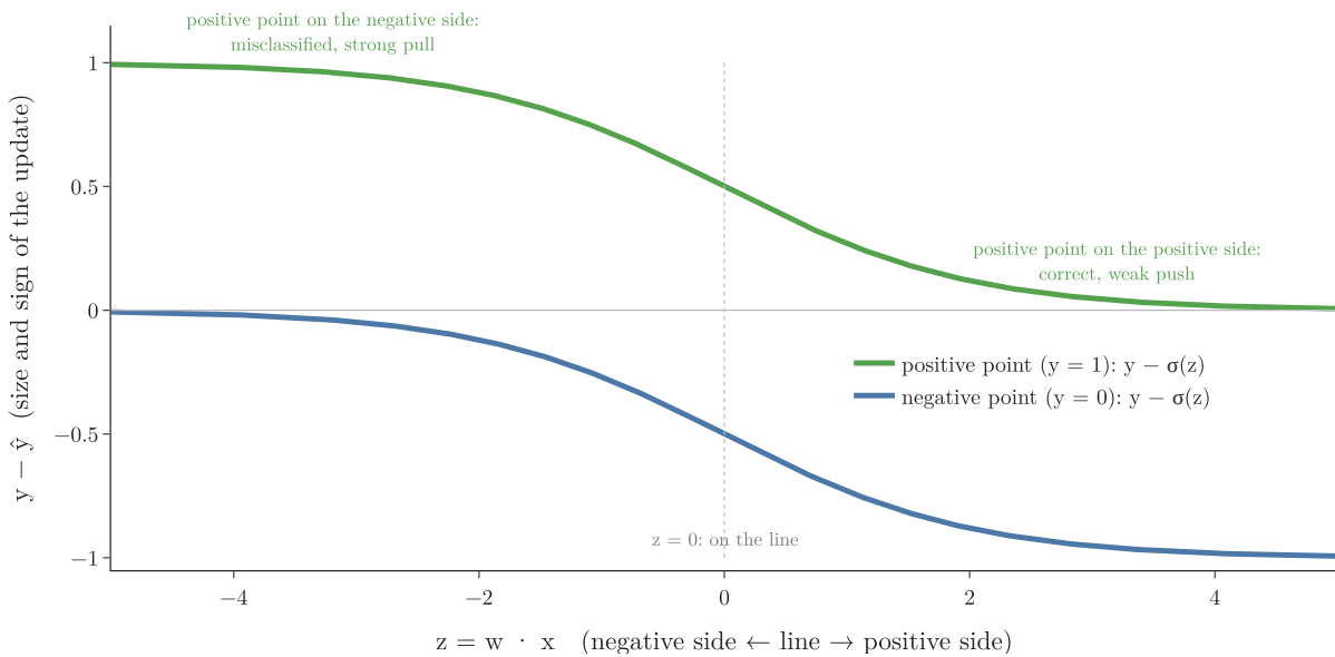
Figure 4: The size of the update against the point's position
