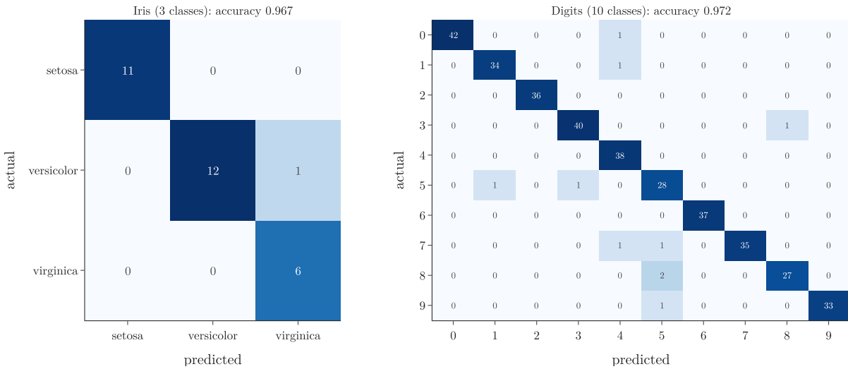
Figure 5: Confusion matrices for iris (3 classes) and digits (10 classes)
