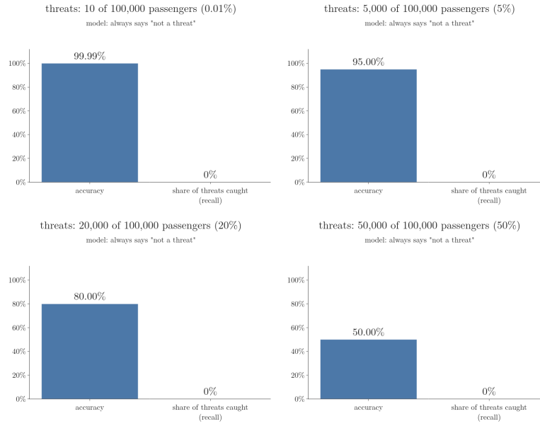
Figure 7: The always-“not a threat” model as the share of threats among 100,000 passengers grows from 0.01 percent to 50 percent. Its accuracy is simply the share of non-threats, so it falls from 99.99 percent to 50 percent. The share of threats it catches stays at 0 throughout
