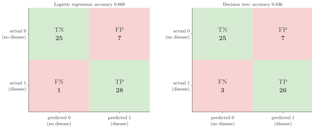
Figure 3: Confusion matrices for logistic regression and the decision tree
