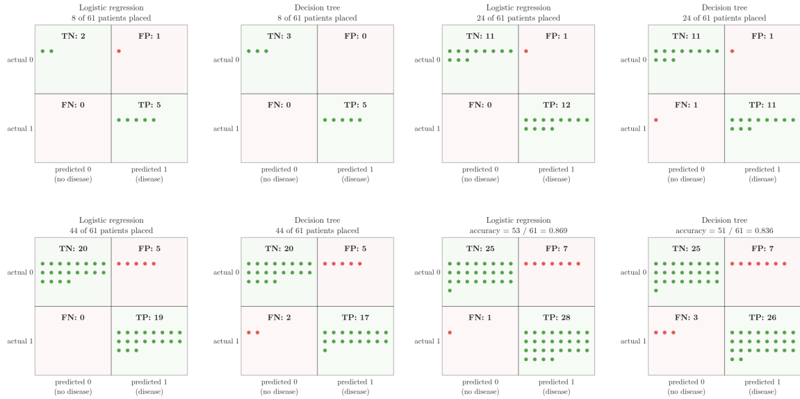
Figure 2: The 61 heart-disease test patients placed one by one into the confusion matrix of each model. Rows are the actual class, columns the predicted class. Green cells (the diagonal) collect the correct predictions, red cells the mistakes. The last frame counts the diagonal: 53 of 61 for logistic regression, 51 of 61 for the decision tree. Colouring the diagonal green and the mistakes red follows StatQuest, “Machine Learning Fundamentals: The Confusion Matrix”; the data and models are our own
