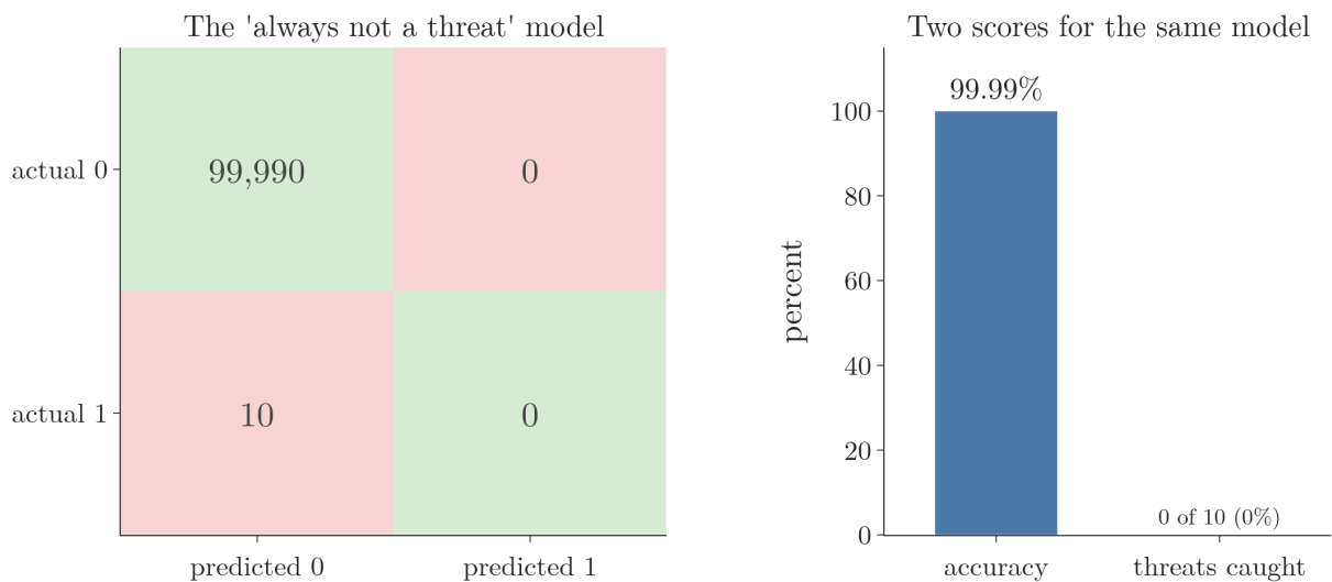
Figure 6: The “always not a threat” model on 100,000 passengers. Left: its confusion matrix. Right: its accuracy against the share of threats it catches.
