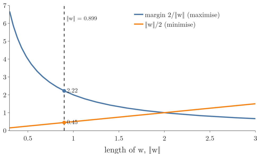
Figure 2: The margin 2/\|w\| (blue) and the term \|w\|/2 (orange) against the length of w . The first falls where the second rises, so the same \|w\| makes the margin largest and the term smallest; marked: \|w\| = 0.899 , margin 2.22, term 0.45.
