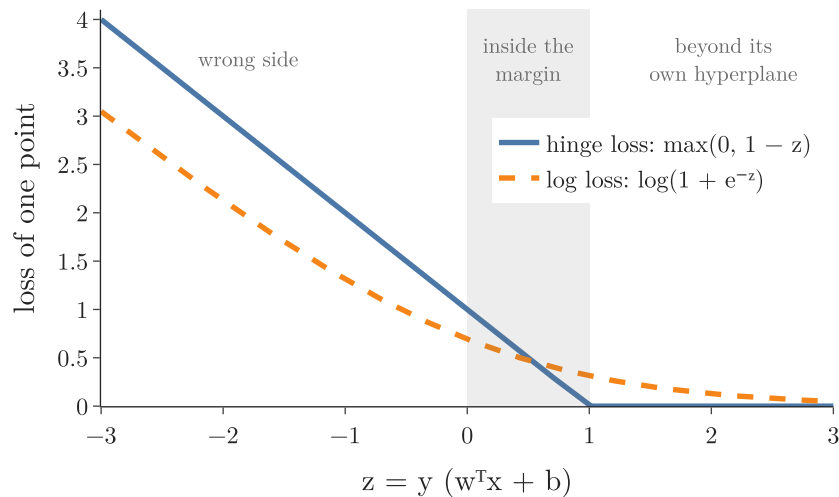
Figure 6: Hinge loss and log loss for one point, against z = y(w^T x + b)
