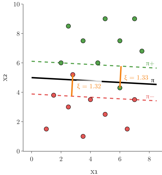
Figure 3: The slack \xi of the two points that break their constraints (orange); all other points have \xi = 0
