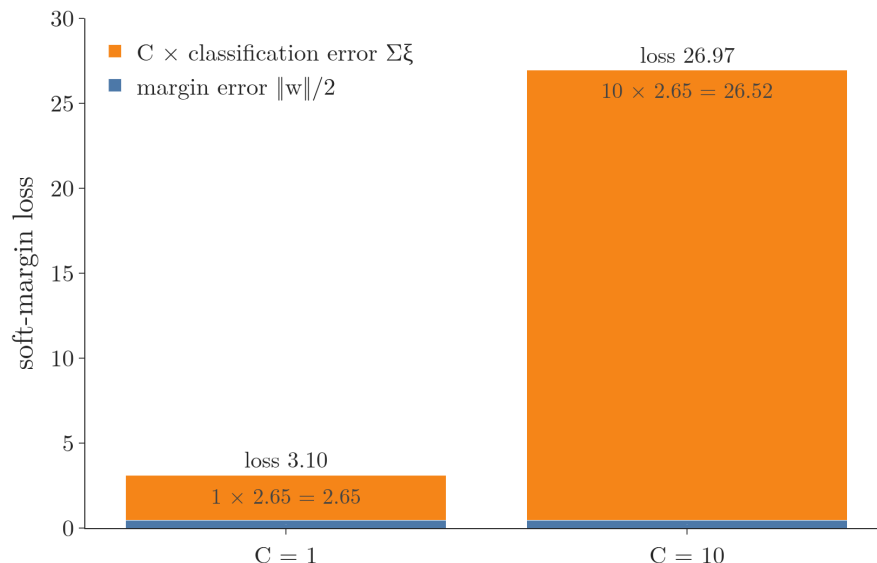
Figure 4: The soft-margin loss of the line of Figure 3 as two stacked parts: margin error 0.45 (blue) and C times the classification error 2.65 (orange). C = 1 gives 3.10; C = 10 gives 26.97.
