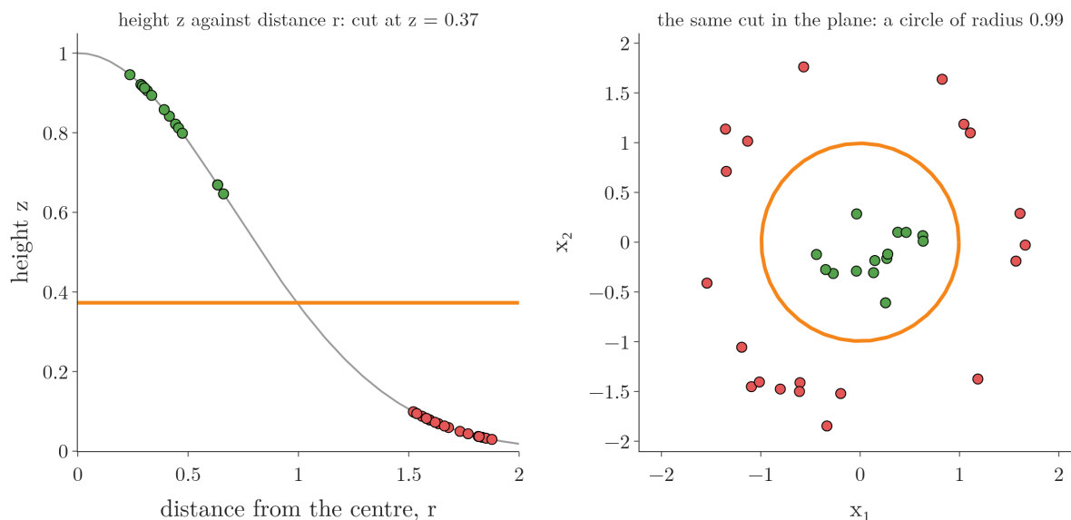
Figure 4: The flat cut of the kernel trick read back in 2D, on the 34 points of Figure 3. Left: height z = \exp(-r^2) against the distance r from the centre, with the cut at z = 0.37 (orange). Right: the same cut in the original plane, a circle of radius 0.99 around the green class.
