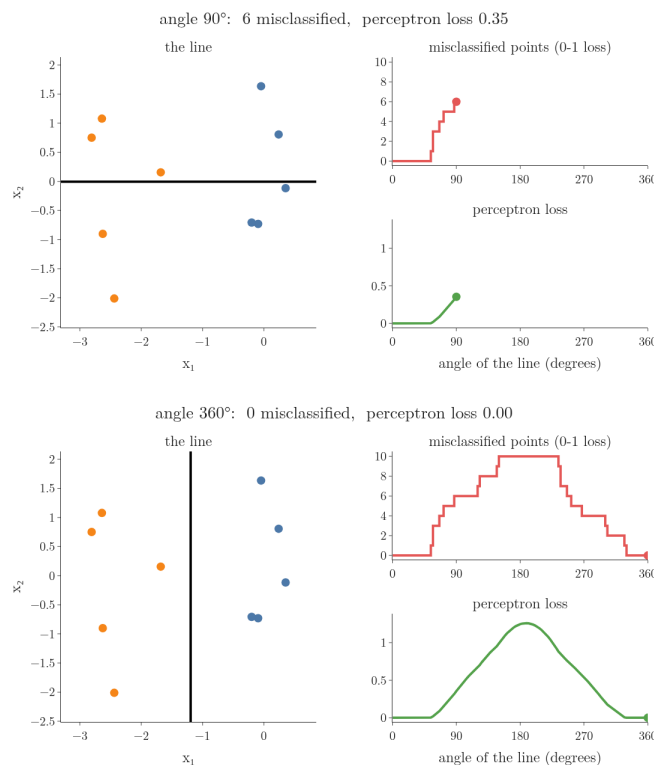
Figure 4: A line turning through 360 degrees over 10 points. Top right: the number of misclassified points (0-1 loss). Bottom right: the perceptron loss, the average of the values of the misclassified points
