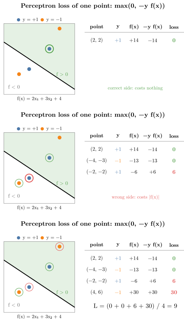
Figure 5: The four cases on the line 2x + 3y + 4 = 0 , one point per case. For each point the row fills in from left to right: the label, the value f(x) , their product with the sign flipped, and the loss
