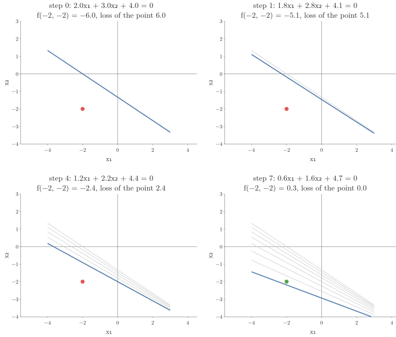
Figure 7: The same step repeated on the point (-2, -2) : each step raises f(-2, -2) by 0.1 \times ((-2)^2 + (-2)^2 + 1) = 0.9 , until the point crosses the line after 7 steps
