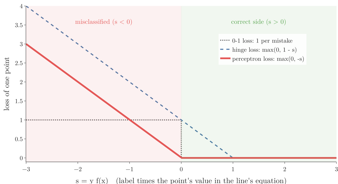
Figure 6: The loss of one point against s = y f(x)
