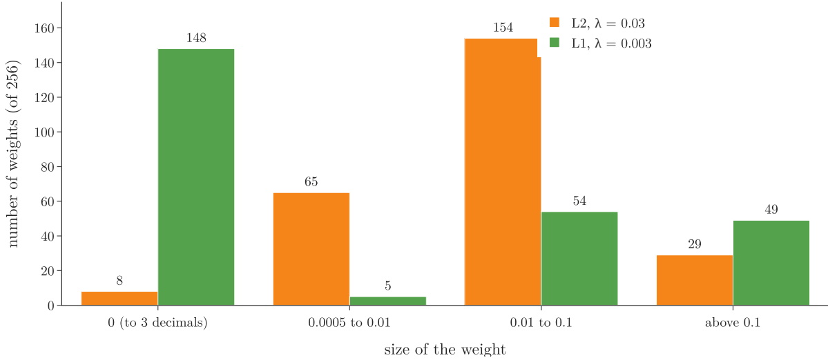
Figure 8: The 256 first-layer weights after 2,000 epochs of plain gradient descent, grouped by size: L2 (orange) and L1 (green), first random start.
