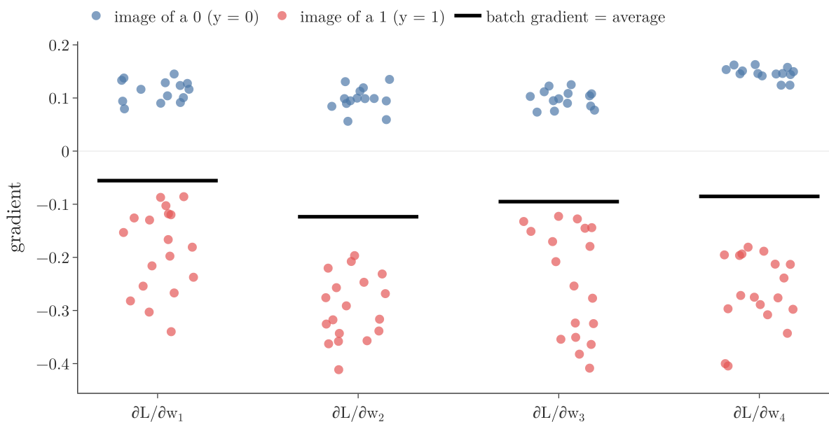
Figure 6: The 32 images of the Notebook’s batch with the starting weights. Each dot is one image’s gradient for one weight of W_2 ; the black bar is the batch gradient, \frac{1}{m}(A_2 - Y)F^\top , their average.
