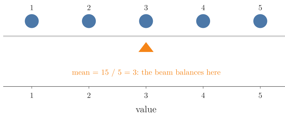
Figure 2: The scores 3, 4, 1, 2, 5 as equal weights on a beam: the mean, 3, is the balance point
