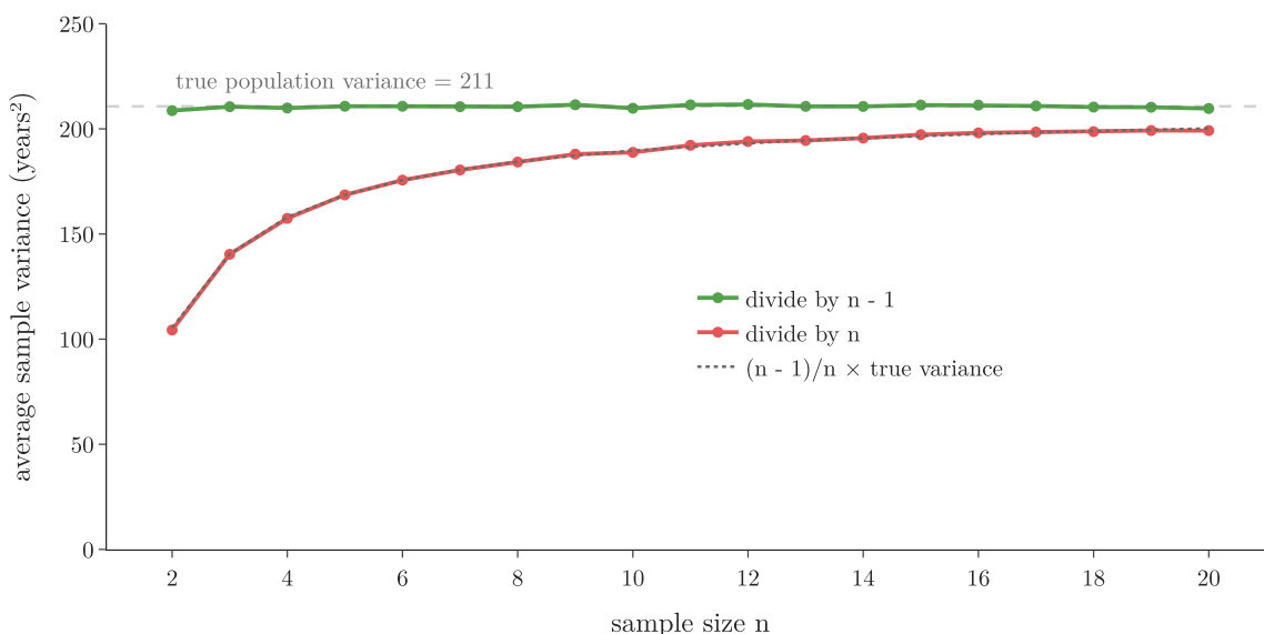
Figure 6: Average sample variance of Titanic ages, dividing by n or by n - 1 ; the dotted curve is (n - 1)/n of the true variance
