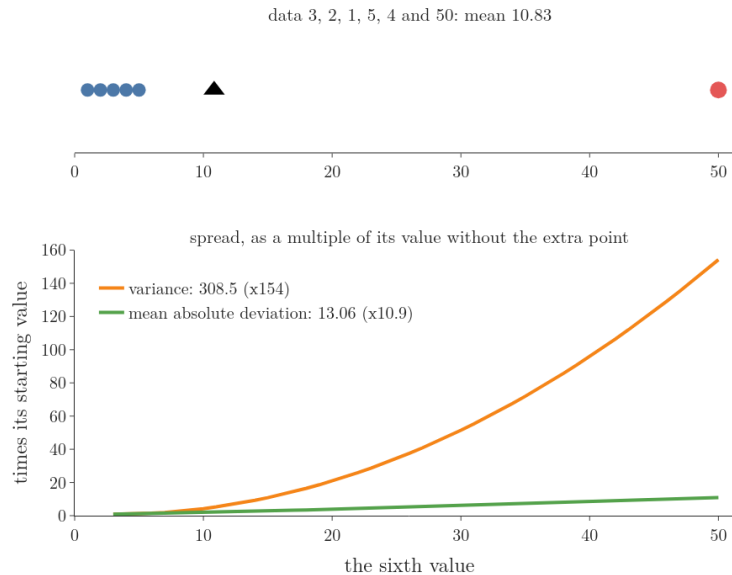
Figure 7: A sixth value moves from 3 to 50: the variance grows with the square of its distance, the mean absolute deviation in proportion
