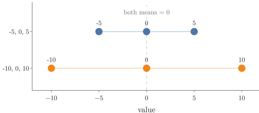
Figure 2: Two features with the same mean, 0, and different spreads
