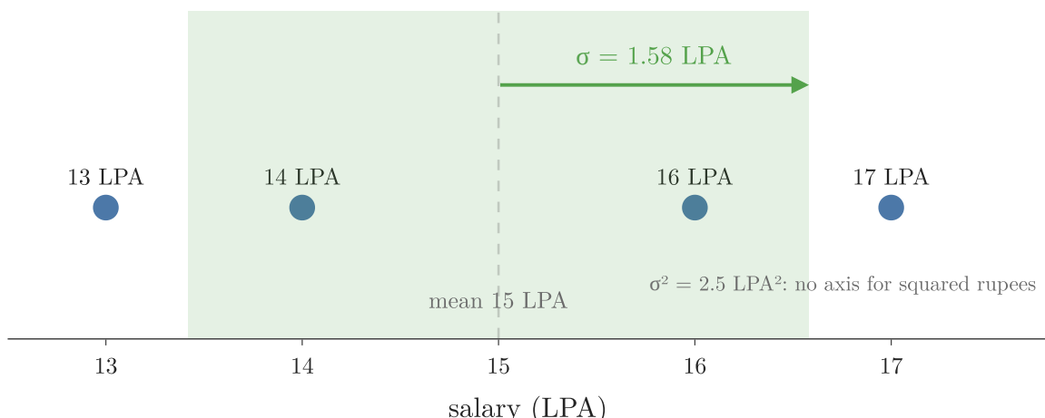
Figure 4: Salaries of 16, 17, 13 and 14 LPA: the standard deviation, 1.58 LPA, is a length on the same axis
