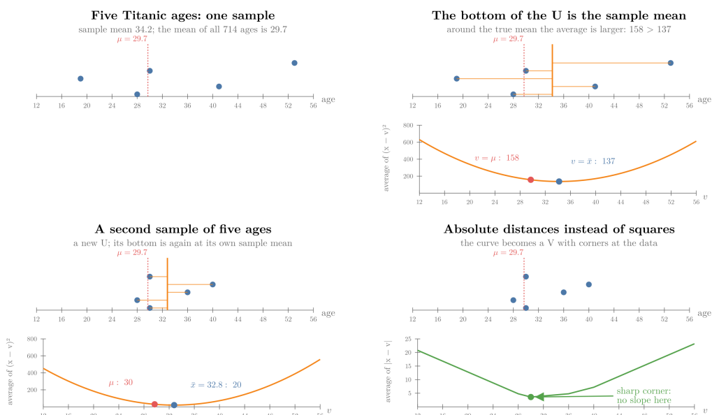
Figure 5: Slide a point v along five ages: the average squared distance to v traces a U whose bottom is the sample mean; a second sample does the same; absolute distances give a V with a sharp corner
