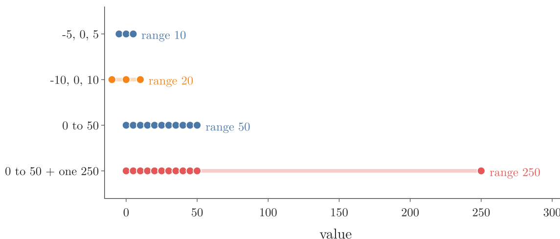
Figure 3: The range of four features: it separates the first two, and one value at 250 stretches the last from 50 to 250
