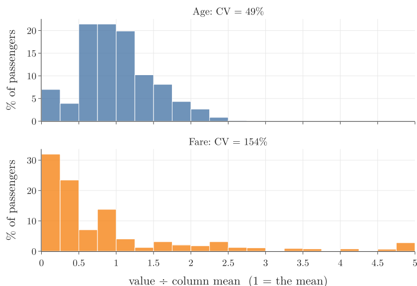
Figure 8: Titanic ages and fares, each divided by its own mean
