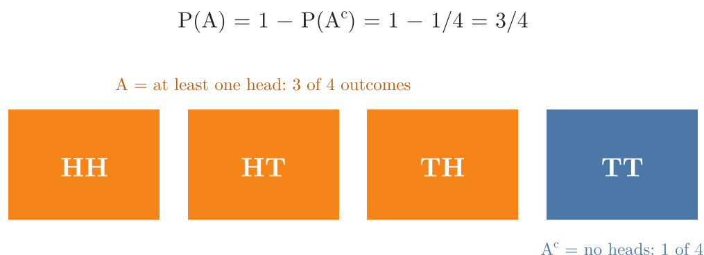
Figure 6: The two-toss sample space split into A = at least one head (orange, 3 outcomes) and its complement, no heads (blue, 1 outcome).
