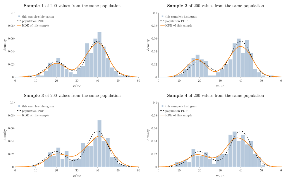
Figure 8: Four samples of 200 values from one two-peaked population. The histogram (bars) changes with every sample; the KDE with bandwidth 3 (orange) stays close to the population PDF (dashed).
