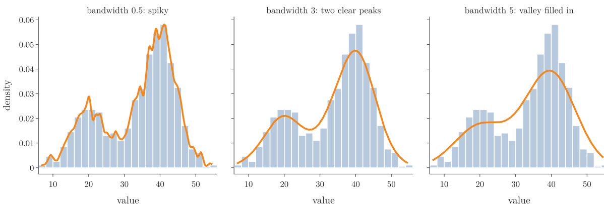
Figure 7: KDE of two-peaked data with bandwidth 0.5, 3 and 5
