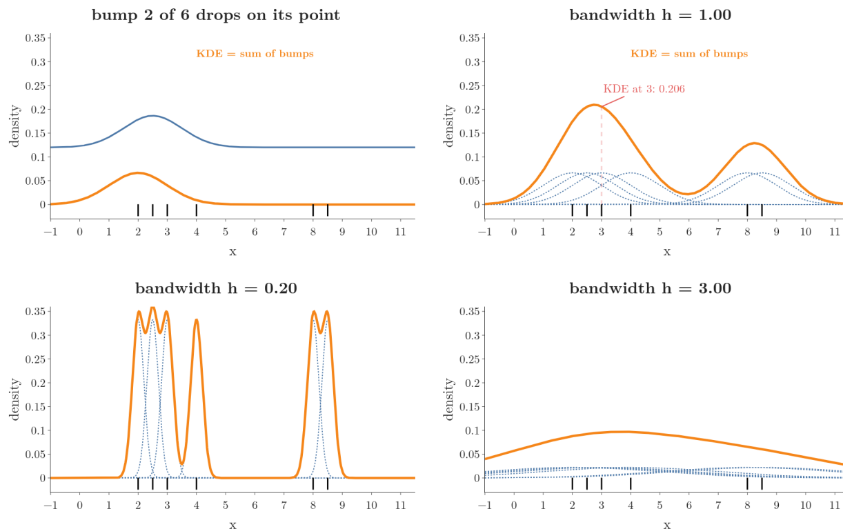
Figure 6: The KDE of section 5.1 built step by step: a bump of bandwidth 1 drops onto each of the six points and the orange sum grows (0.206 at x = 3 ). Then the bandwidth sweeps from 0.2 (six spikes) to 3 (one hill)
