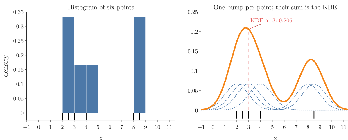
Figure 5: KDE by hand: a Gaussian bump of bandwidth 1 on each of six points (dotted); their scaled sum is the KDE (orange)
