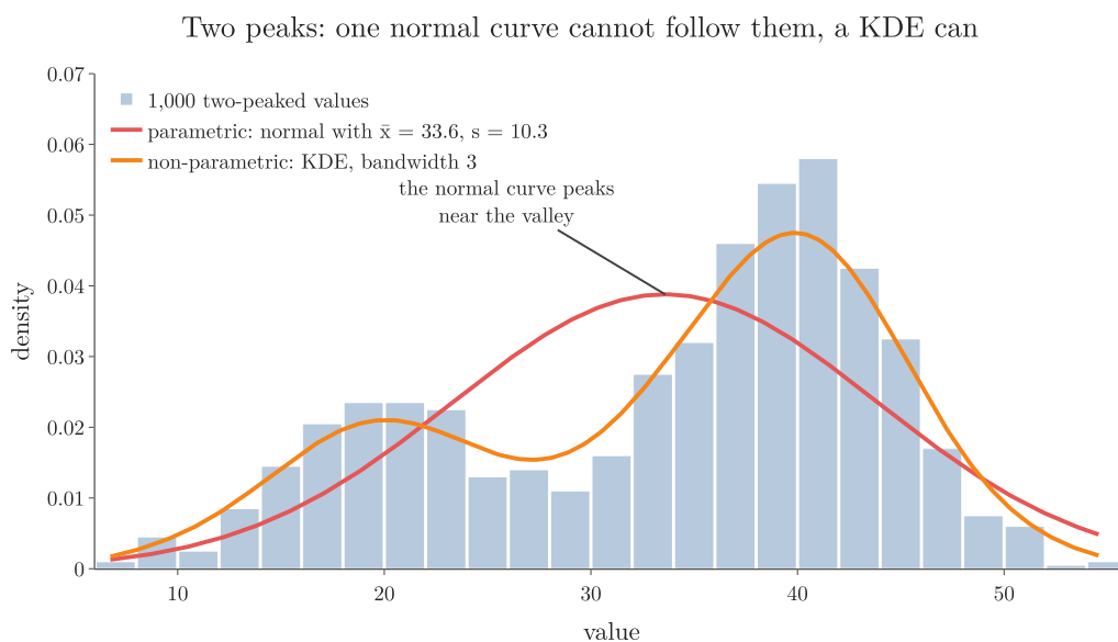
Figure 4: 1,000 two-peaked values. Red: the fitted normal PDF, one hump centred between the groups. Orange: the KDE with bandwidth 3, which follows both peaks.
