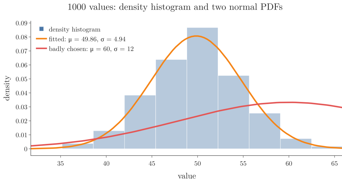
Figure 2: 1,000 values: the density histogram, the fitted normal PDF and a normal PDF with badly chosen parameters
