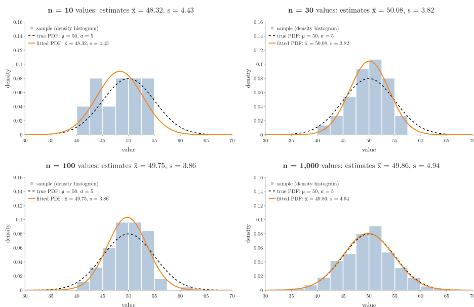
Figure 3: Normal PDFs fitted to the first 10, 30, 100 and 1,000 values of the sample (orange) against the true PDF with mean 50 and standard deviation 5 (dashed).
