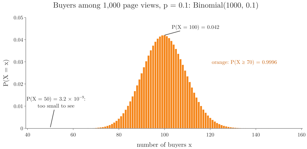
Figure 6: The PMF of the number of buyers among 1,000 page views with p = 0.1 . The peak is P(X = 100) = 0.042 ; P(X = 50) is invisible; the orange bars, 70 and above, hold 0.9996 of the probability.
