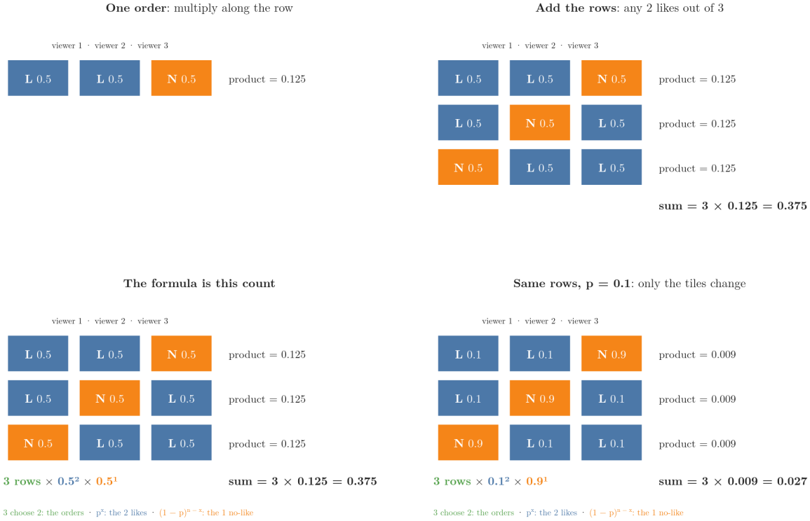
Figure 5: The three orders of 2 likes among 3 viewers. Each row multiplies to 0.125 and the rows add to 0.375; the formula’s three pieces are the number of rows, the like tiles and the no-like tile. With p = 0.1 the same rows give 3 \times 0.009 = 0.027 . Idea after StatQuest, “The Binomial Distribution and Test, Clearly Explained!!!”.
