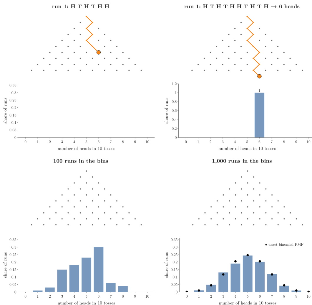
Figure 8: A Galton board for 10 fair-coin tosses: each ball is one run of 10 Bernoulli trials and lands in the bin of its head count. The bins fill with the 1000 runs above; the dots are the exact binomial PMF. Idea after Sanderson (3Blue1Brown), “But what is the Central Limit Theorem?”
