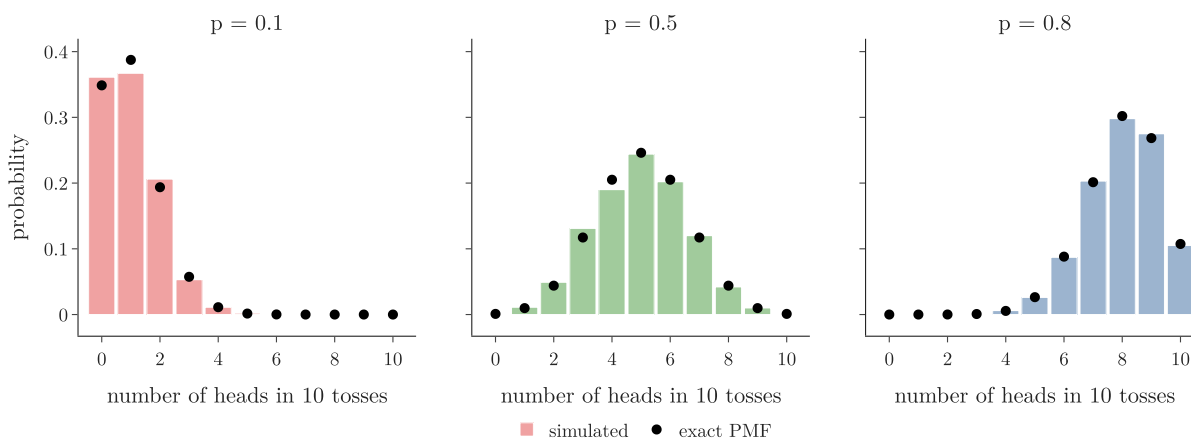
Figure 9: 1000 simulated runs of 10 tosses (bars) against the exact binomial PMF (dots)
