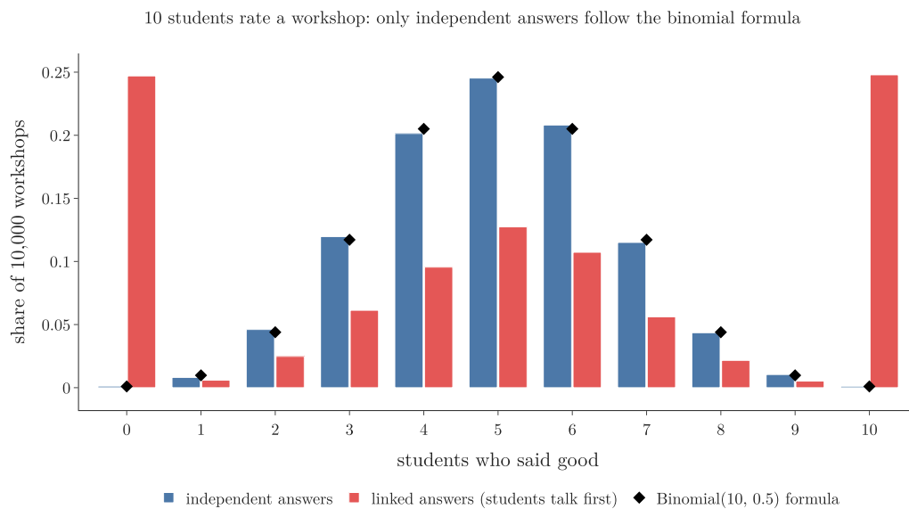
Figure 7: 10,000 simulated workshops of 10 students. Blue: independent answers, matching the Binomial(10, 0.5) formula (diamonds). Red: linked answers, which pile up at 0 and 10.
