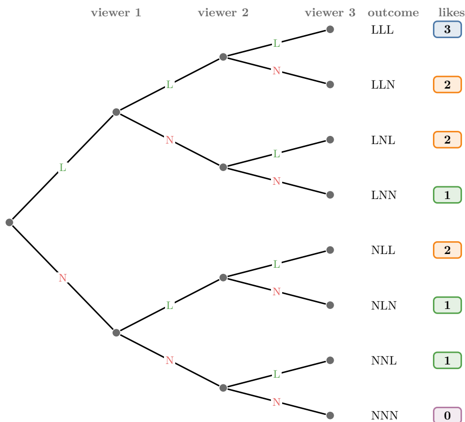
Figure 4: Every outcome for three viewers and the number of likes in each
