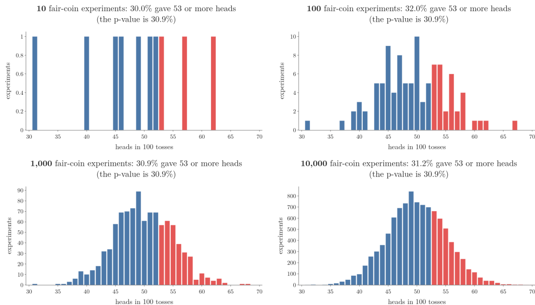
Figure 3: 10 to 10,000 simulated experiments of 100 fair-coin tosses. Red: experiments with 53 or more heads; their share settles near the p-value, 30.9%.
