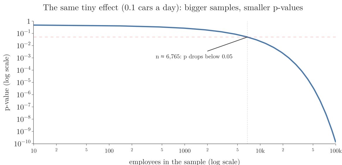
Figure 4: The p-value of the right-tailed z-test at a true effect of 0.1 cars a day ( \sigma = 5 ), for samples of 10 to 100,000 employees. The effect never changes; only the sample size does.
