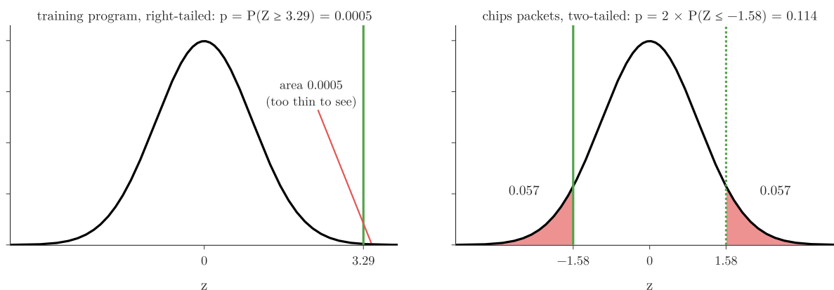
Figure 7: P-values (red areas) of the two z-tests
