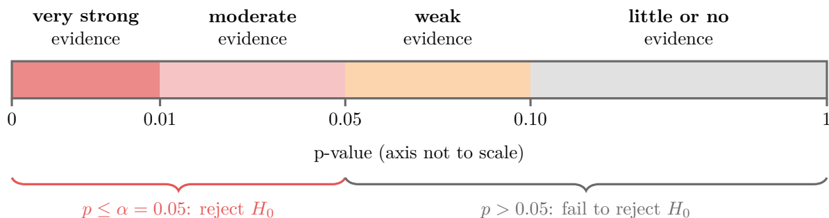
Figure 6: A common rule of thumb for reading p-values
