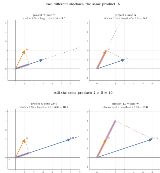
Figure 3: Both views on Section 2’s vectors: the shadows differ, the products agree (5), and after stretching \mathbf{v} to 2\mathbf{v} both give 10
