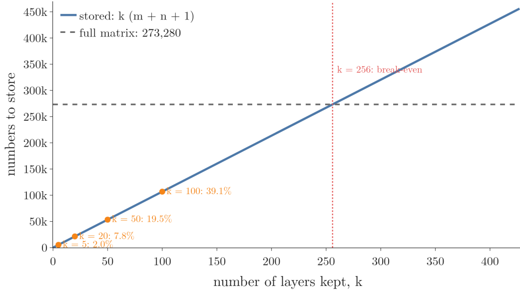
Figure 5: The numbers stored for a rank- k approximation of the 427 \times 640 photo, k(m + n + 1) , against the 273,280 numbers of the full matrix. k = 20 needs 7.8%; from k = 256 on, the layers cost more than the matrix.
