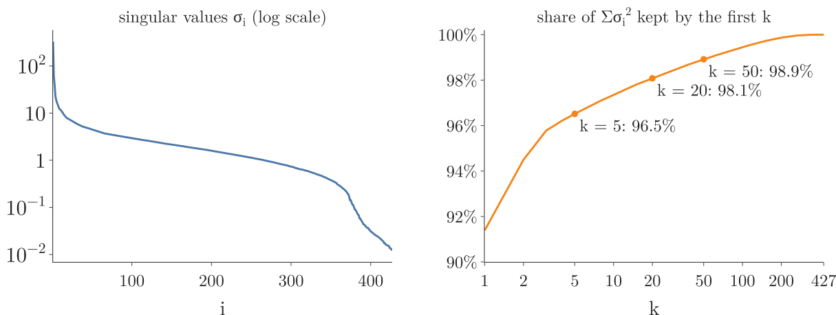
Figure 9: Singular values of the photo, and the share of \sum \sigma_i^2 kept by the first k
