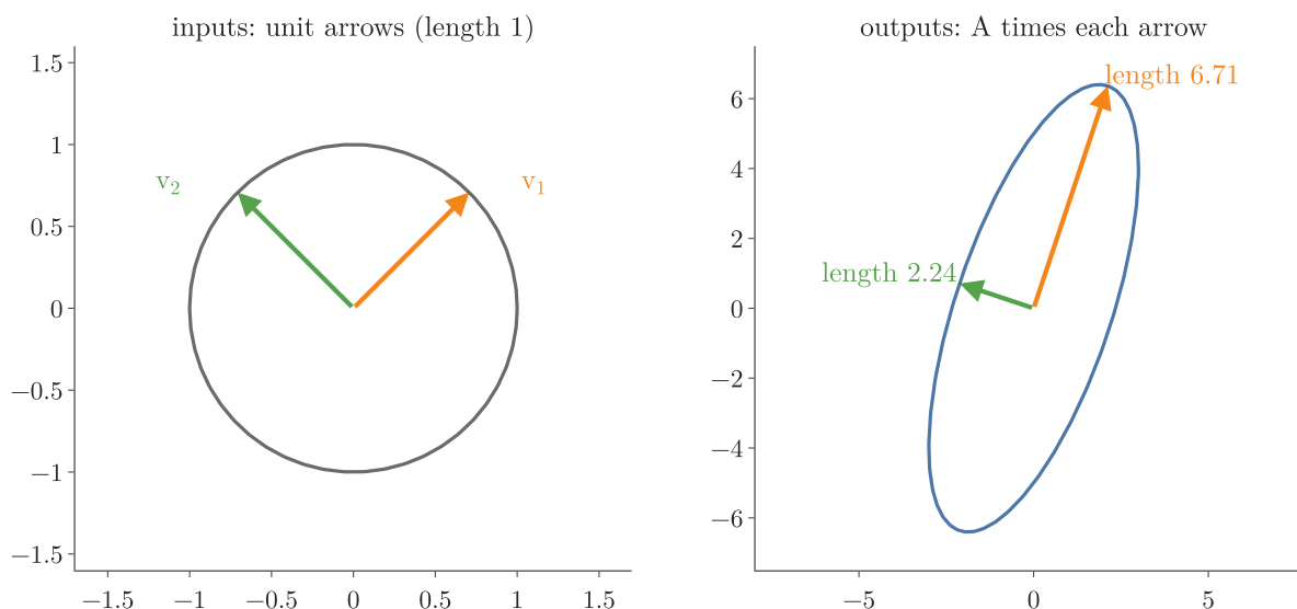
Figure 6: Left: arrows of length 1 end on the unit circle; two of them, v_1 and v_2 , are drawn. Right: the matrix A sends the circle to an ellipse; v_1 comes out longest, 6.71, and v_2 shortest, 2.24
