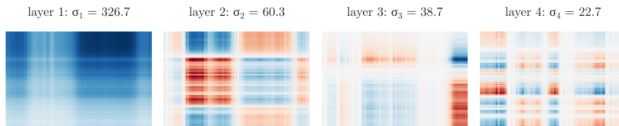
Figure 4: The first four layers \sigma_i \mathbf{u}_i \mathbf{v}_i^T of the photo: blue positive, red negative, white zero
