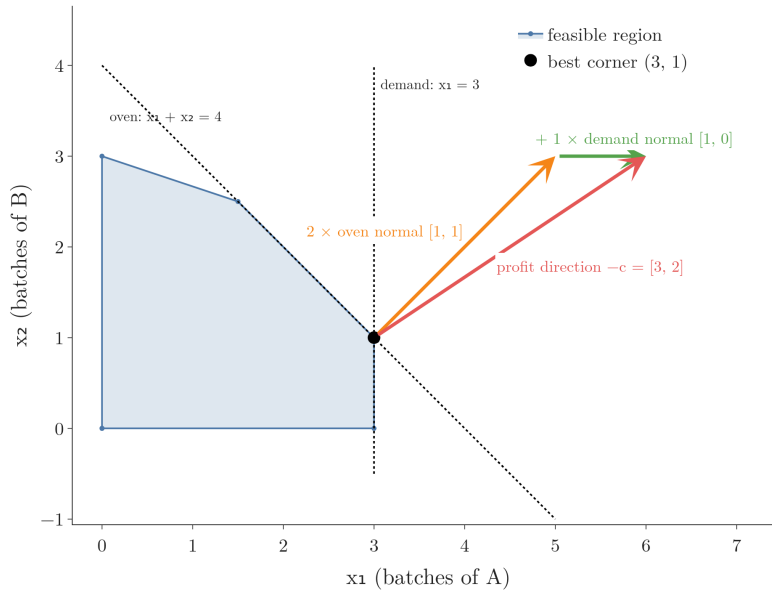
Figure 4: The dual condition at the best corner (3, 1) . The profit direction -\mathbf{c} = [3, 2] (red) equals 2 times the oven normal [1, 1] (orange) plus 1 times the demand normal [1, 0] (green): non-negative weights, the multipliers 2 and 1.
