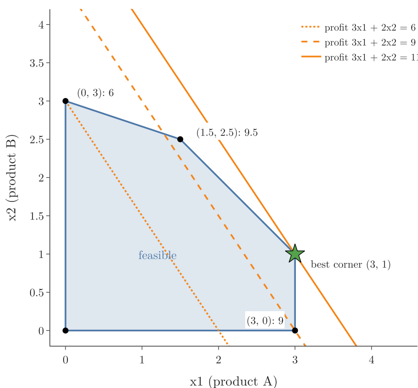
Figure 1: A linear program: the feasible region (blue) is a polygon, and the profit lines 3x_1 + 2x_2 = 6, 9, 11 slide outward until the last one touches the region at a corner, (3,1)
