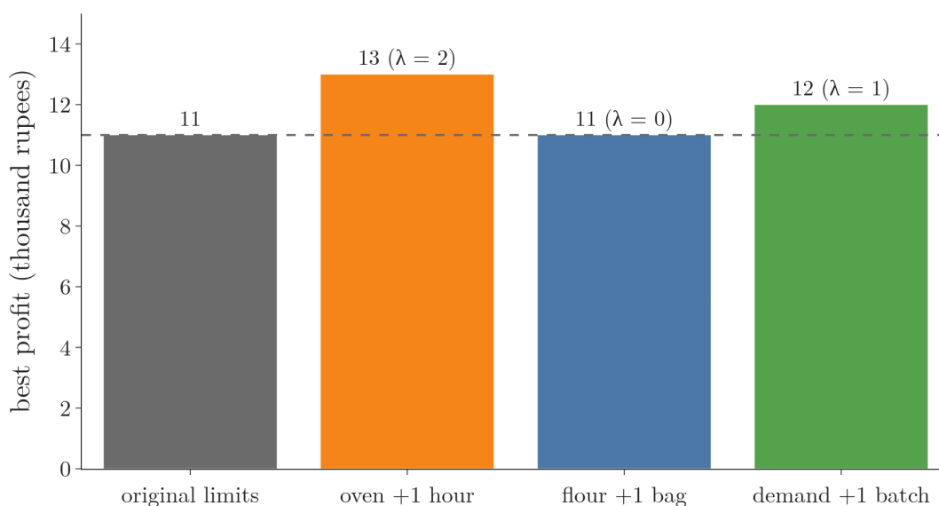
Figure 5: The best profit re-solved with one more unit of each resource. Oven: 13, up by 2. Flour: 11, unchanged. Demand: 12, up by 1. The rises are the multipliers.
