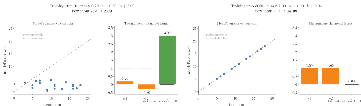
Figure 4: Training a model on 20 pairs of numbers and their sums. Left: each dot is one pair, the model’s answer against the true sum. Right: the three parameters, with black marks at 1, 1 and 0.
