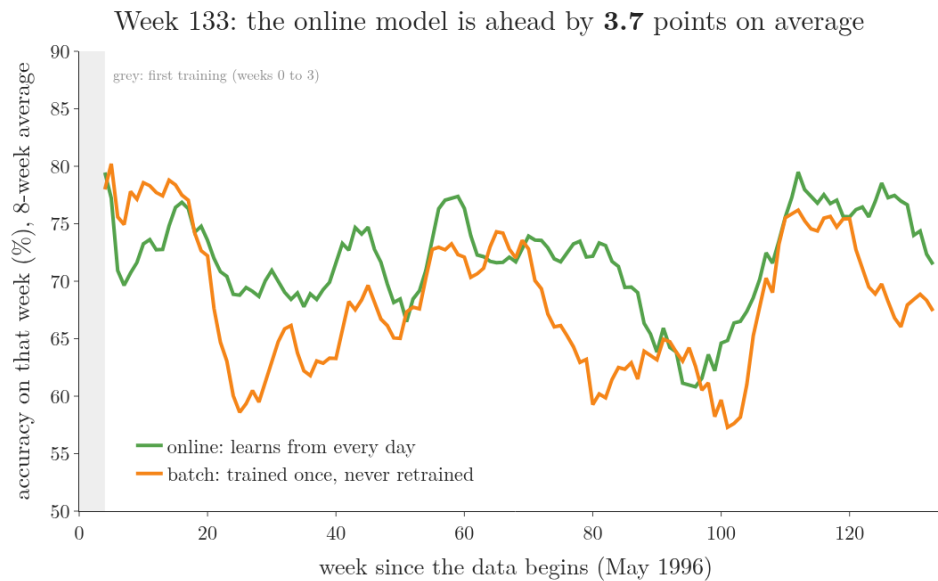
Figure 4: Online vs batch on the Electricity market data. Orange: a batch model trained once on the first 4 weeks. Green: an online model that starts from the same 4 weeks, then each day predicts that day’s 48 half hours, and then learns from their true answers with one small update. Accuracy on each week, averaged over 8 weeks.
