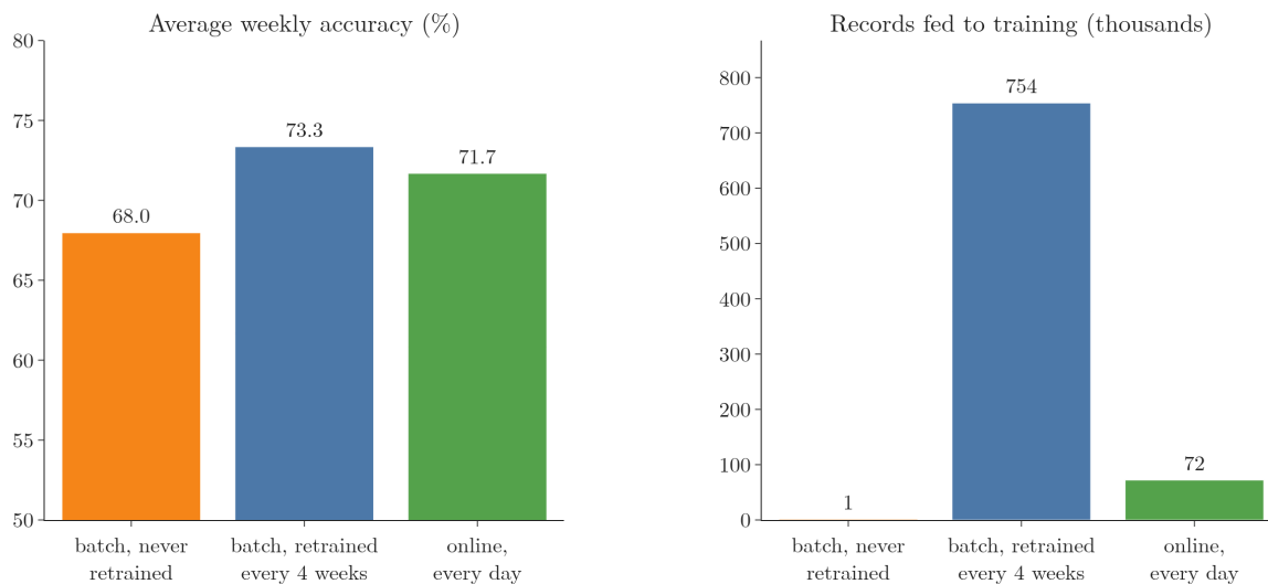
Figure 9: Accuracy against training work on the Electricity market data, weeks 4 to 133. Training work counts each record once each time it is fed to training.
