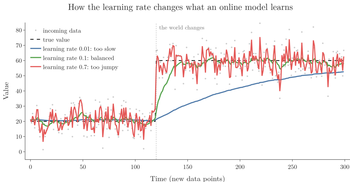
Figure 6: How the learning rate changes what an online model learns (simulation)
