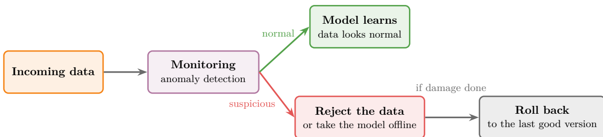
Figure 8: Protecting an online model
