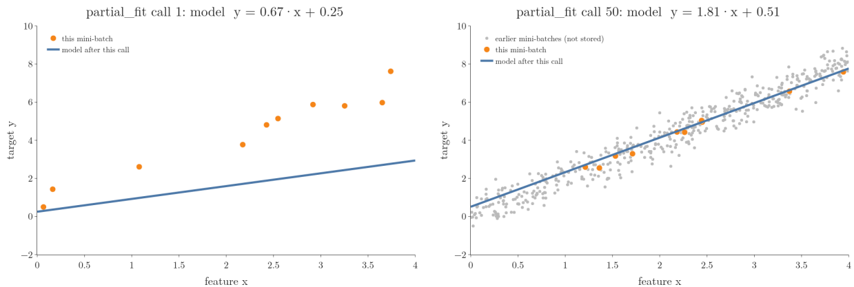
Figure 5: An SGDRegressor learning from a stream with partial_fit . Orange: the mini-batch of this call. Grey: earlier mini-batches, which the model has already used and does not keep. Blue: the model’s line after the call.
