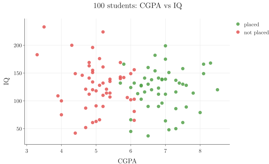
Figure 2: CGPA vs IQ, coloured by placement
