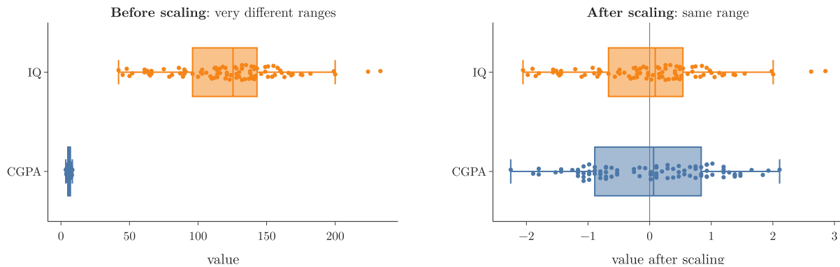
Figure 5: CGPA and IQ before and after scaling
