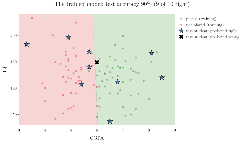
Figure 7: What the trained model learned
