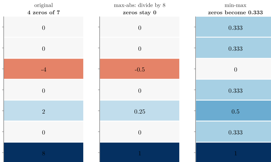
Figure 7: A sparse column (left), the same column after max-abs scaling (zeros stay 0) and after min-max scaling (every zero becomes 0.333).
