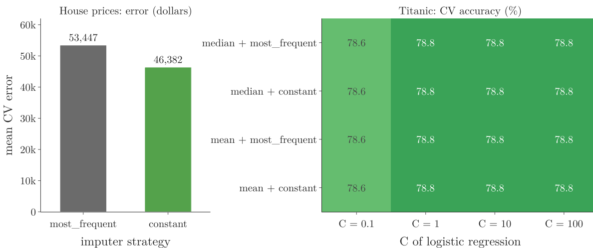
Figure 11: Grid search results: on house prices the “Missing” category clearly wins; on the Titanic pipeline all four imputer combinations tie and only C matters
