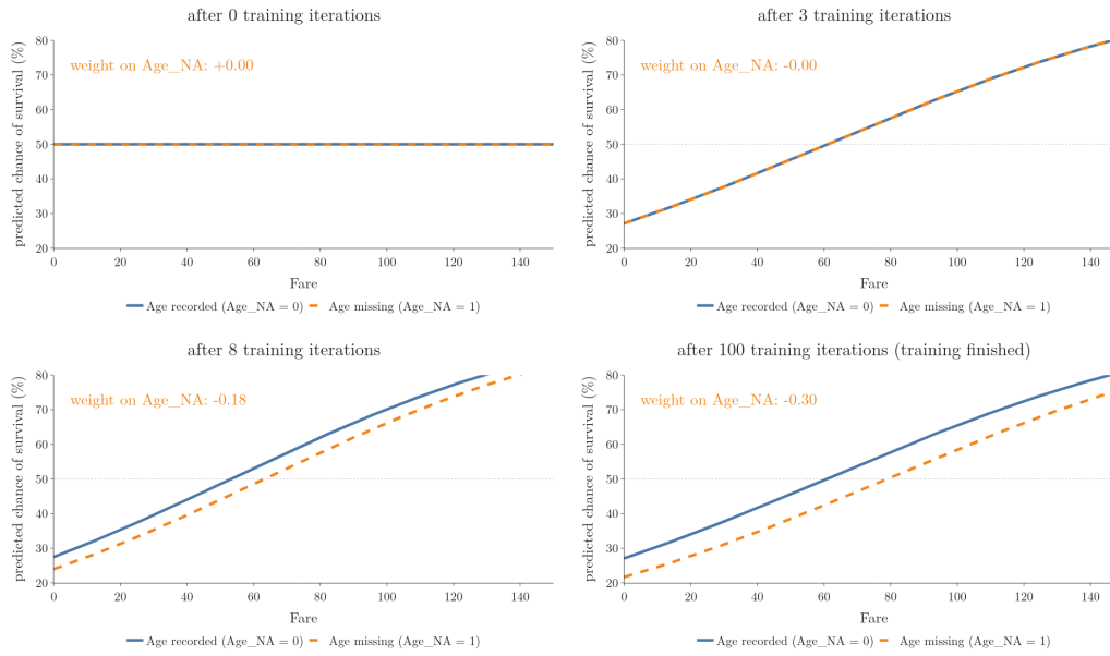
Figure 9: The model of Section 6.3 during training: the curves for \text{Age\_NA} = 0 and \text{Age\_NA} = 1 start as one and separate as the coefficient of \text{Age\_NA} moves from 0 to -0.30
