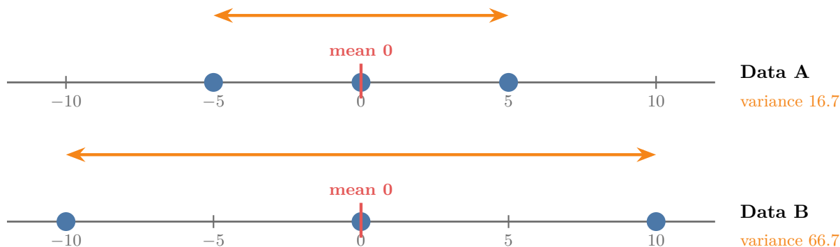
Figure 6: Same mean, different spread
