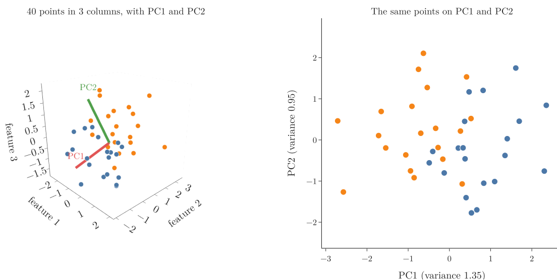
Figure 8: The 40 points in 3D with PC1 and PC2, and after projection
