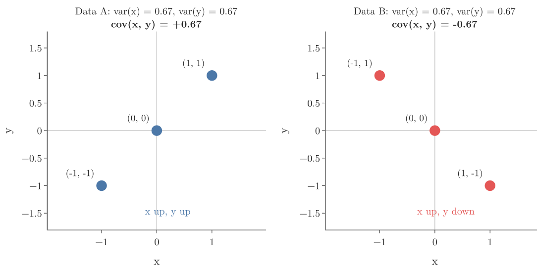
Figure 3: Same variances, opposite covariance
