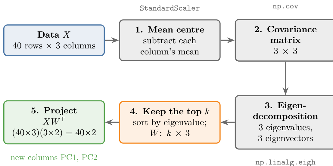
Figure 7: PCA step by step
