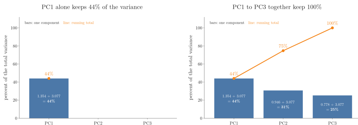
Figure 9: The scree plot of the 3-feature example, built one component at a time. Bars: eigenvalue \div sum of eigenvalues. Orange line: the running total.
