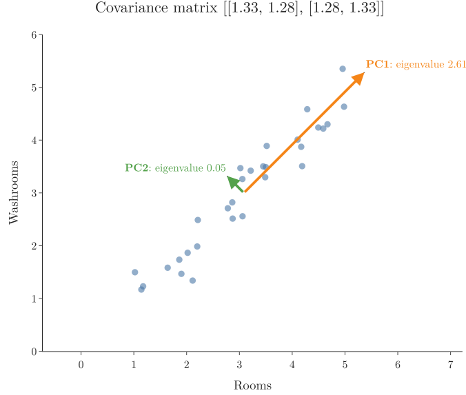
Figure 6: The eigenvectors of the covariance matrix of the flats data
