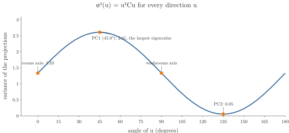
Figure 2: The variance of the projections of the 30 flats for every direction u , from 0 to 180 degrees. The maximum, 2.61 at 45 degrees, is PC1; the minimum, 0.05 at 135 degrees, is PC2.
