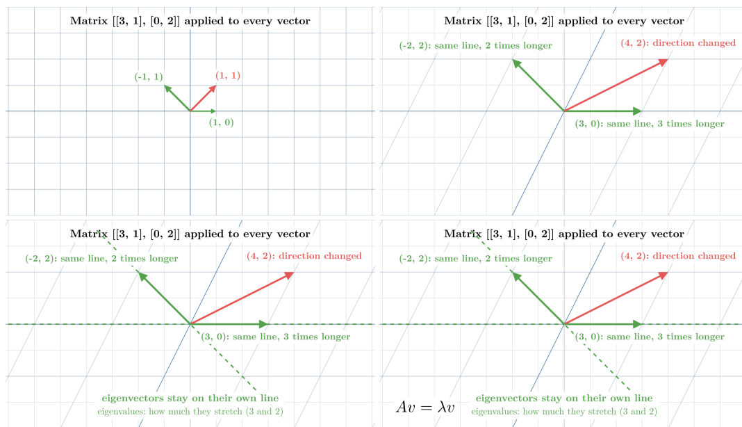
Figure 5: Applying a matrix: most vectors turn, eigenvectors only stretch. Idea and matrix after 3Blue1Brown, “Eigenvectors and eigenvalues”.
