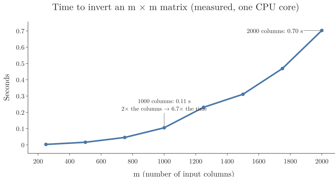
Figure 8: Time to invert a matrix as its size grows
