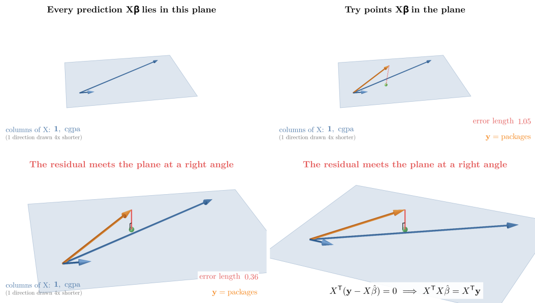
Figure 7: The column space of X for three students is a plane (the two blue columns span it). The target y (orange) sticks out of it. Moving the prediction X\beta through the plane, the error length is smallest, 0.36, at the foot of the perpendicular from y , where the residual meets the plane at a right angle
