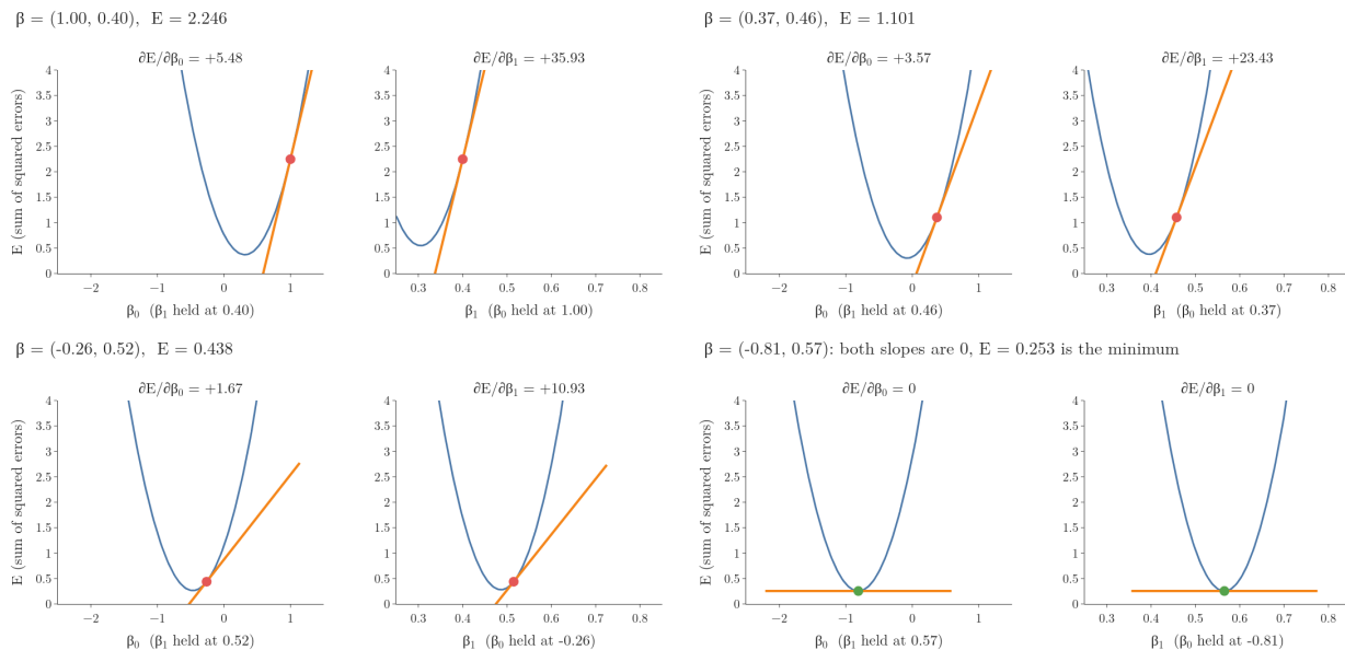
Figure 5: The gradient -2X^T y + 2X^T X\beta on the four students: each panel is the error E along one coefficient, the orange tangent's slope is one entry of the gradient, and both reach 0 together at \beta = (-0.81, 0.57)
