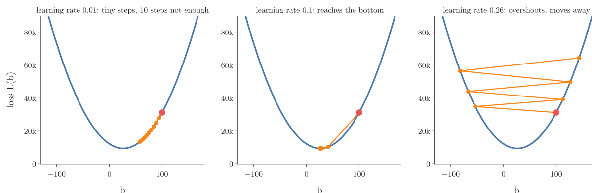
Figure 5: Three learning rates from the same start
