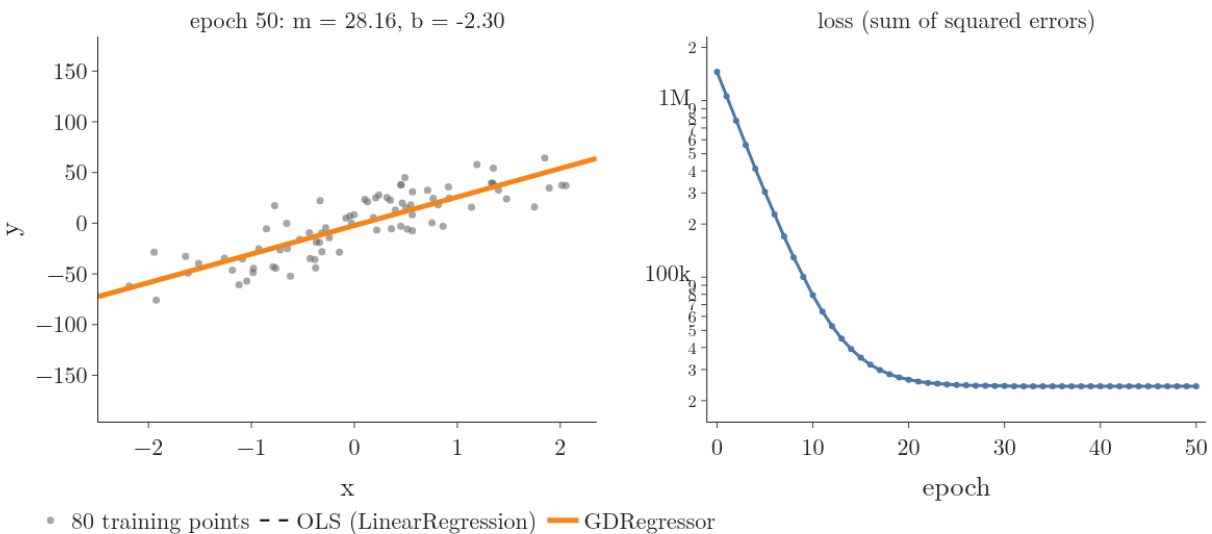
Figure 7: The GDRegressor class at work on the 80 training points: the line after each epoch (orange) closing in on the OLS line (dashed), and the loss per epoch on a log scale.
