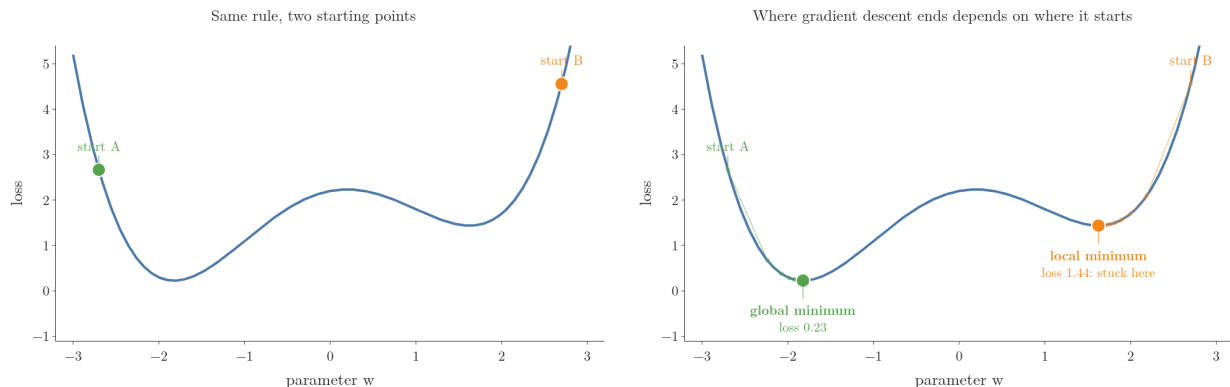
Figure 9: Two runs of gradient descent on the same non-convex curve (learning rate 0.07). Start A reaches the global minimum; start B stops in the local minimum. The ball-rolling picture follows 3Blue1Brown, “Gradient descent, how neural networks learn”.
