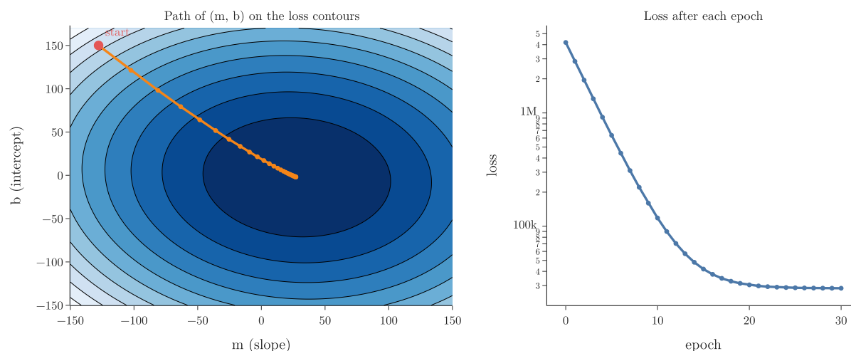
Figure 6: Gradient descent on m and b : the path and the loss per epoch
