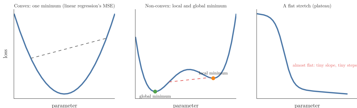
Figure 8: Convex and non-convex loss functions
