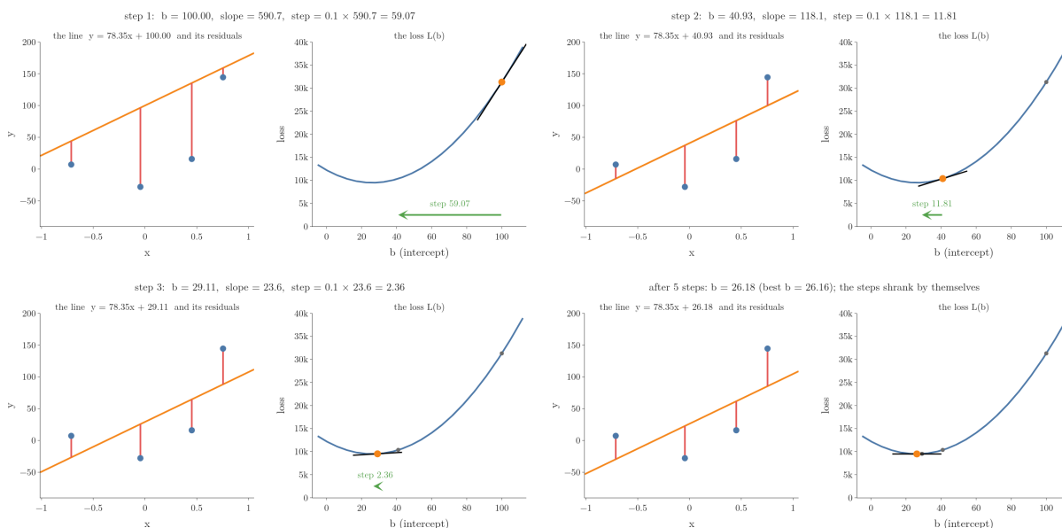
Figure 4: Gradient descent on b , seen on the data (left) and on the loss curve (right). Each frame prints b , the slope and the step. Idea after StatQuest, “Gradient Descent, Step-by-Step”.
