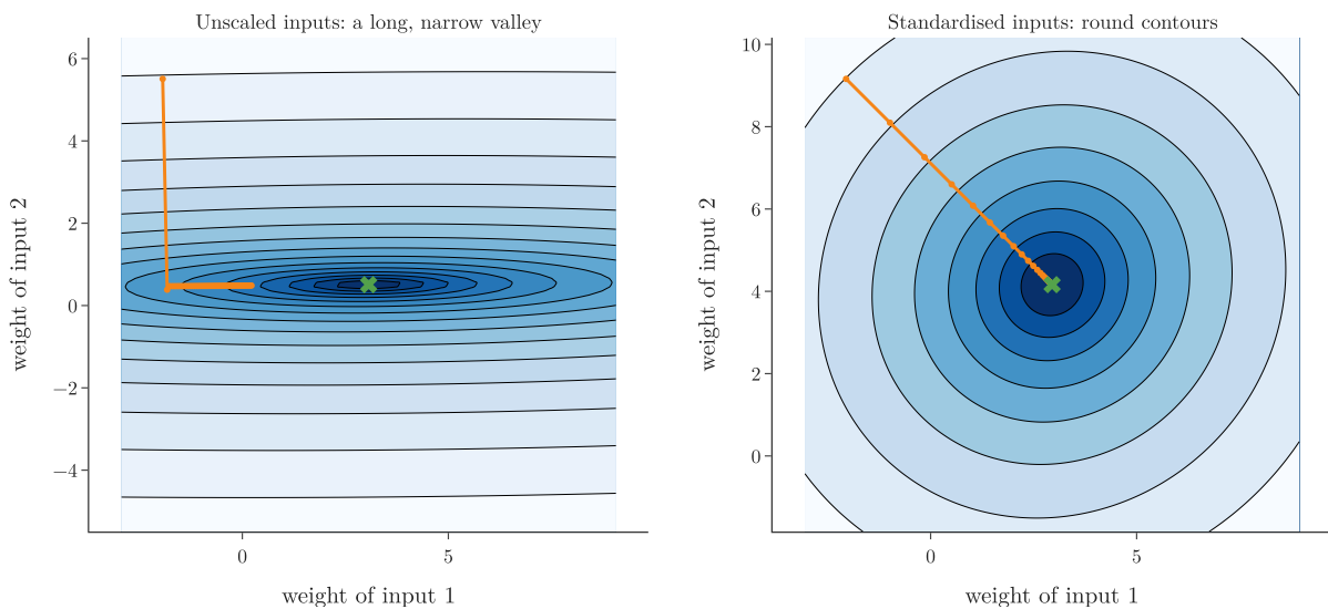
Figure 10: The effect of scaling the inputs on gradient descent
