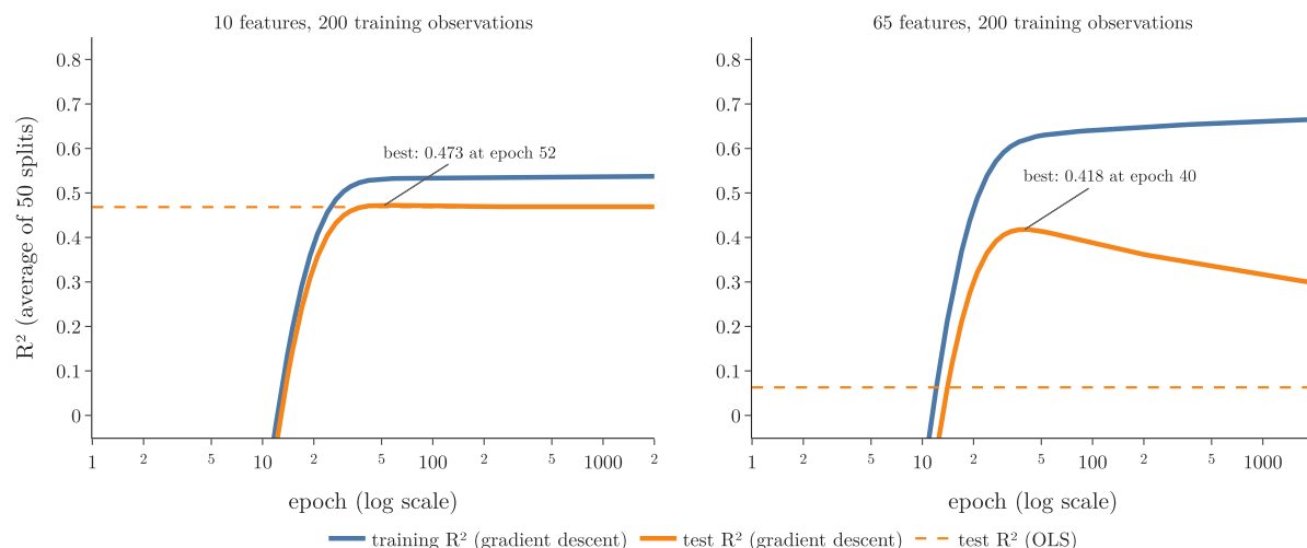
Figure 5: Training and test R^2 over the epochs, averaged over 50 random splits. Left: 10 features, where gradient descent ends at the OLS value. Right: 65 features, where test R^2 peaks early and then falls towards OLS.
