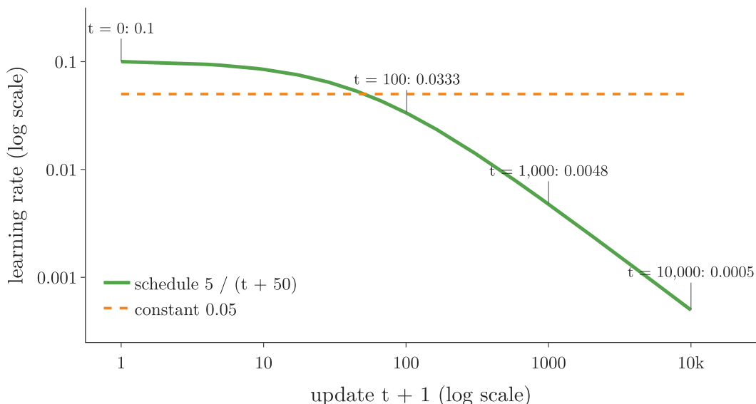
Figure 6: The learning schedule 5 / (t + 50) against a constant rate of 0.05, both axes on a log scale
