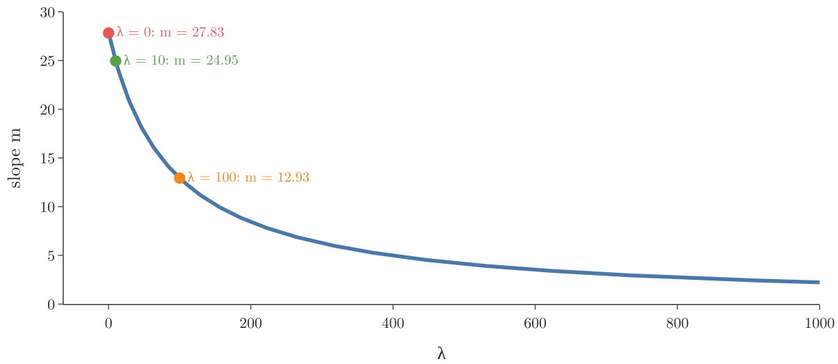
Figure 3: The Ridge slope against \lambda
