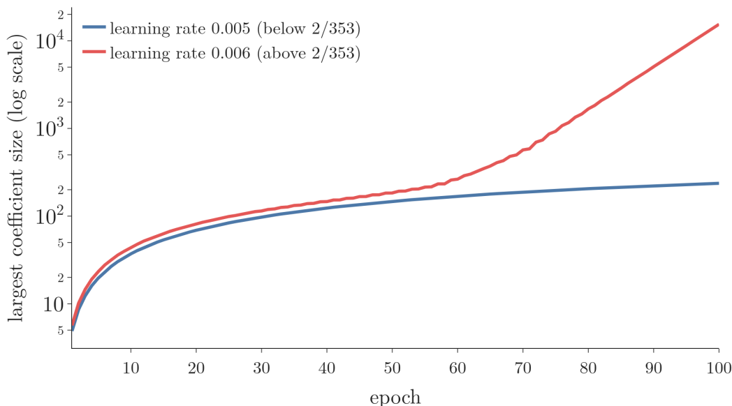
Figure 5: The largest coefficient of the from-scratch code per epoch on the diabetes data, alpha 0.001. Learning rate 0.005 (blue, below the limit 2/353 ) settles; 0.006 (red, above it) grows to about 15,000 after 100 epochs. Log scale.
