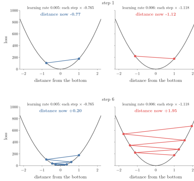
Figure 4: One direction of the loss bowl, curvature 353. Left: learning rate 0.005, each step multiplies the distance from the bottom by -0.765 , so the jumps shrink. Right: learning rate 0.006, each step multiplies it by -1.118 , so the jumps grow
