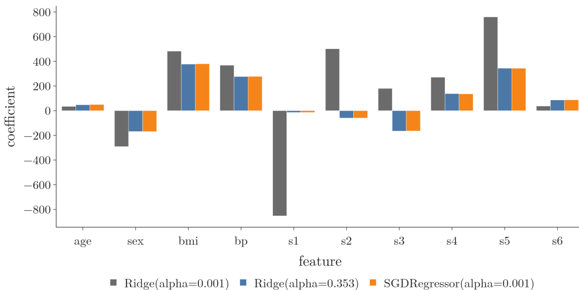
Figure 7: Coefficients on the diabetes training data (353 observations): Ridge with \alpha 0.001 (grey) and 0.353 (blue), and SGDRegressor with \alpha 0.001 run for 50,000 epochs (orange). The orange bars match the blue ones.
