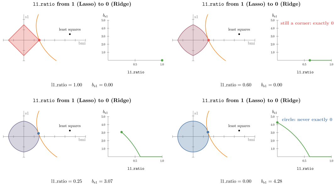
Figure 5: The feasible region morphs from Lasso’s diamond ( l1_ratio 1) to Ridge’s circle ( l1_ratio 0) on two diabetes features. The s1 coefficient, where the loss ellipse first touches the region, stays exactly 0 down to l1_ratio 0.6 and then grows to 4.28
