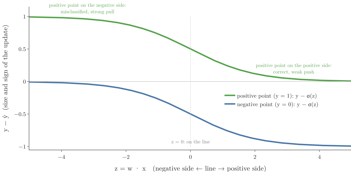
Figure 6: The size of the update against the point's position
