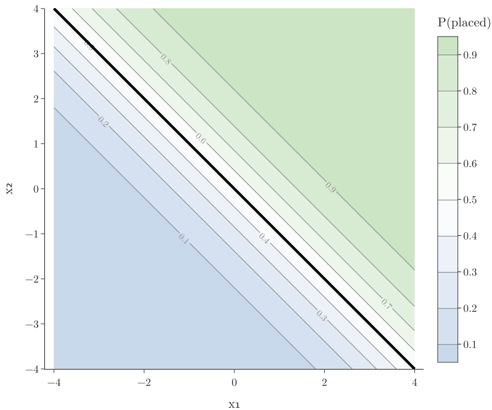
Figure 4: \sigma(w \cdot x) as the probability of being placed
