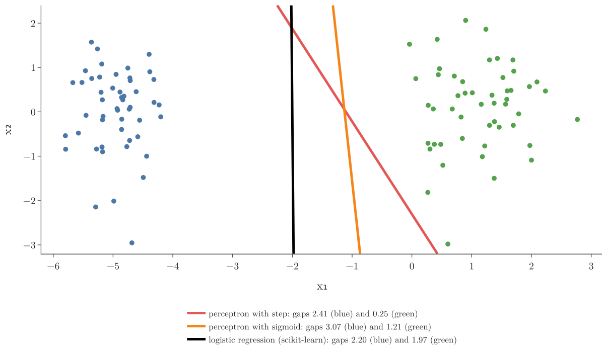
Figure 8: Step perceptron, sigmoid perceptron and logistic regression
