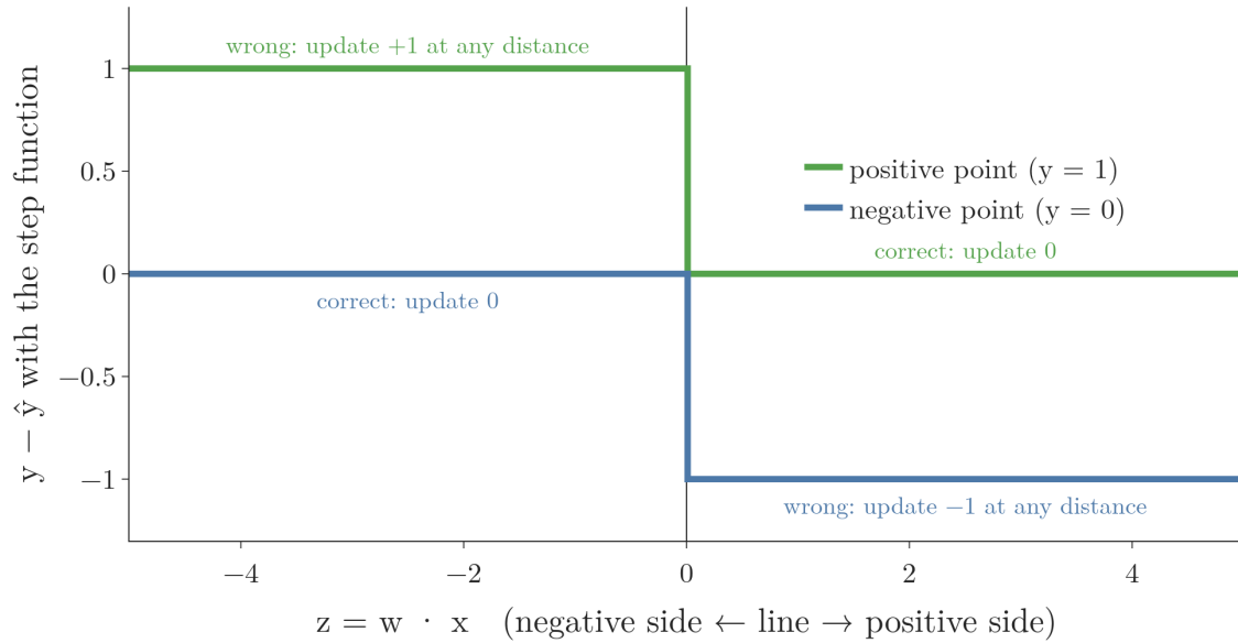
Figure 1: The update y - \hat{y} with the step function, against the point's position z = w \cdot x . Correct points give 0 at any distance; wrong points give +1 (positive points, green) or -1 (negative points, blue) at any distance.
