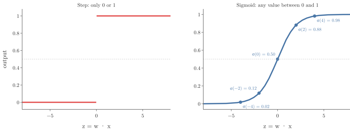
Figure 2: The step function and the sigmoid function
