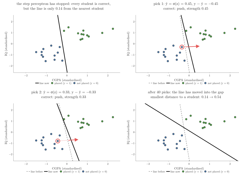
Figure 7: The sigmoid rule on 24 students, starting from the line where the step perceptron stopped (dashed in the last frame). Each frame: the picked student (ring) pushes the line away; the arrow's length is the strength |y - \hat{y}| . Near students push hard, far students gently. After 40 picks the smallest distance from the line to a student has grown from 0.14 to 0.54.
