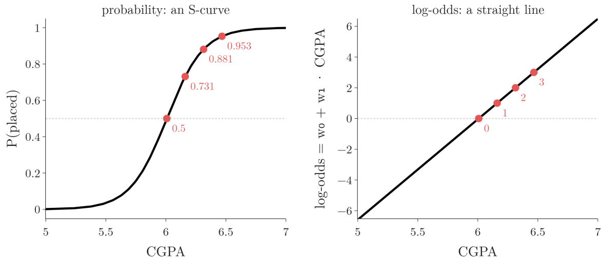
Figure 5: The fitted CGPA model drawn two ways. Left: the probability of being placed, an S-curve. Right: the log-odds, a straight line. The red points mark the same four CGPA values in both panels: probabilities 0.5, 0.731, 0.881 and 0.953 are log-odds 0, 1, 2 and 3.
